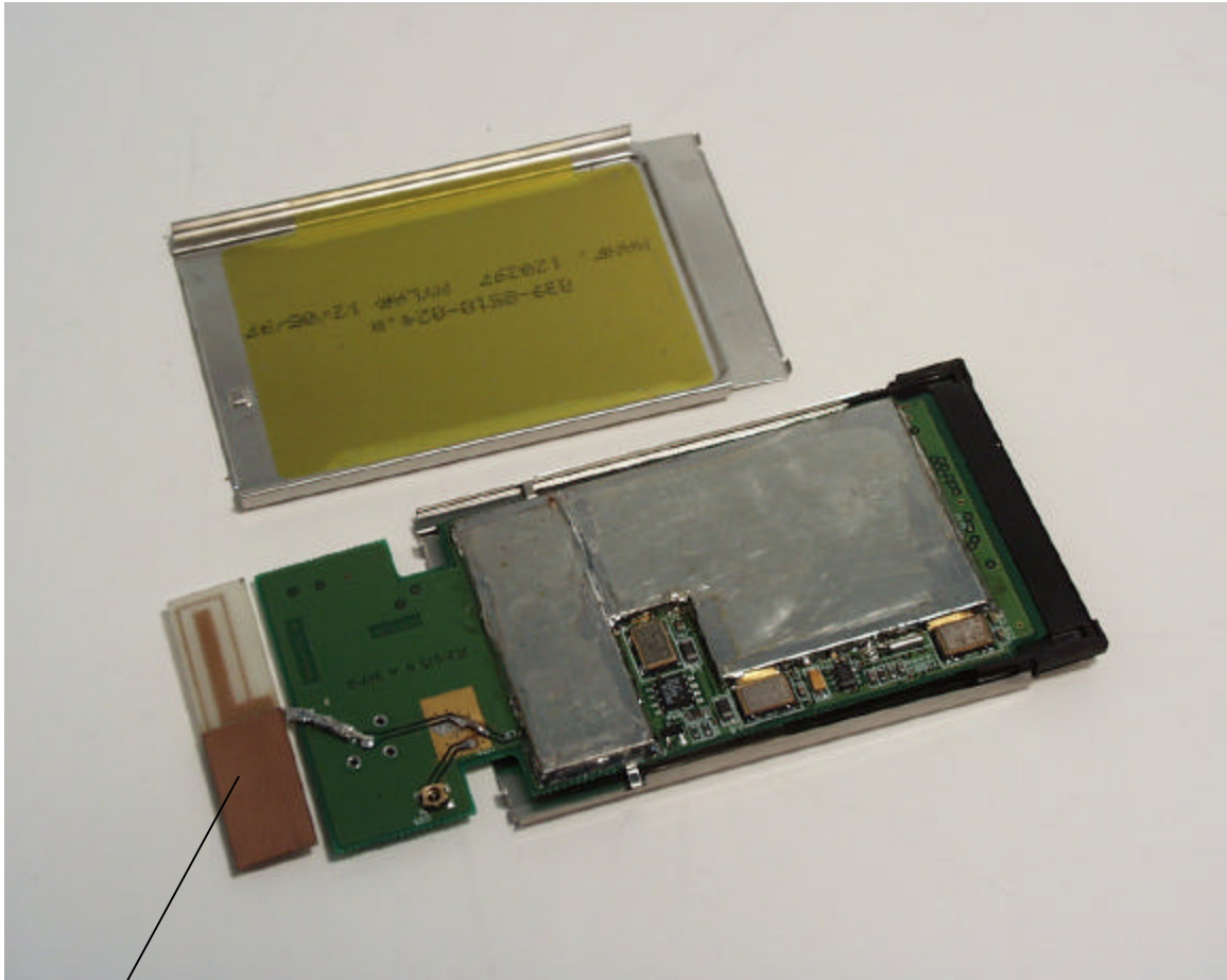
Antenna element
