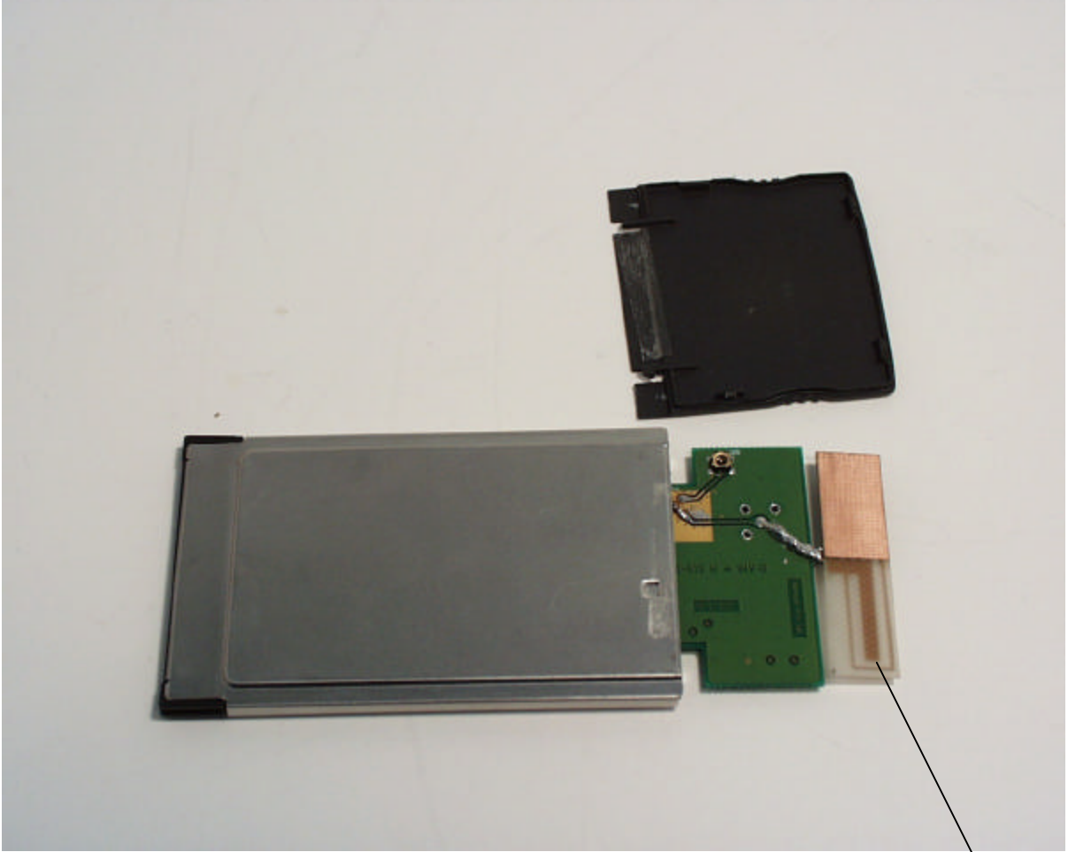
Antenna element
