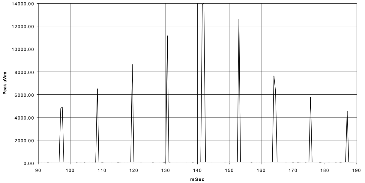
Fine Tune Pulses, 288MHz fundamental Linear Scale
