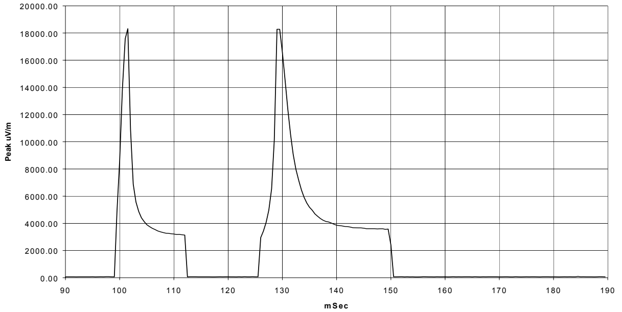
Coarse Tune Pulses, 310MHz fundamental Linear Scale
