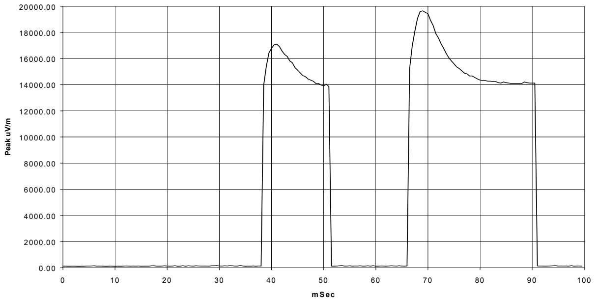
Coarse Tune Pulses, 418MHz fundamental Linear Scale
