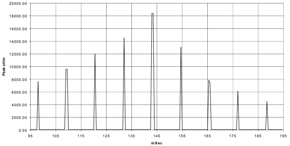
Fine Tune Pulses, 310MHz fundamental Linear Scale
