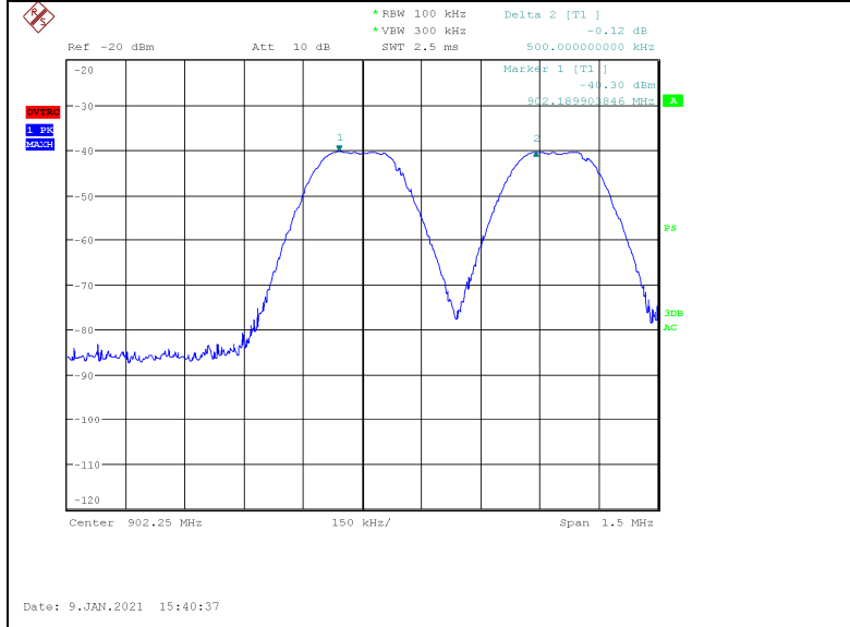
Channel Separation Low Band Measurement Plot
