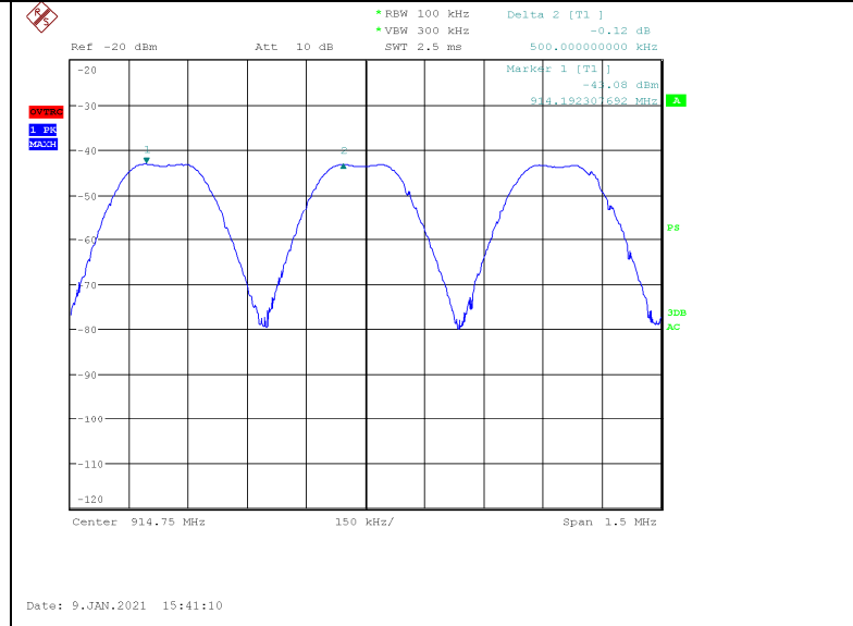
Channel Separation Mid Band Measurement Plot
