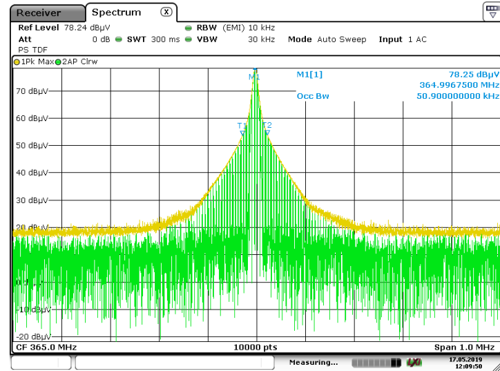
Measuring Occupied Bandwidth at -20dB points
