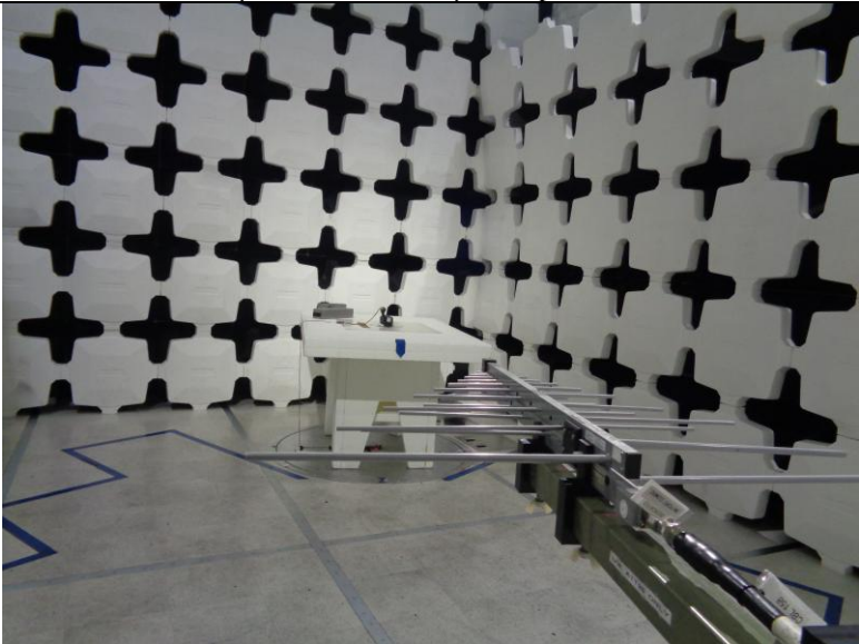
LPA (200-1000MHz) Setup Overview
