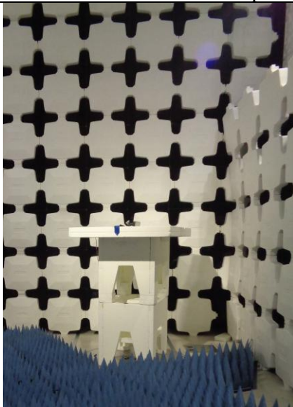
LPA (200-1000MHz) Setup Overview
