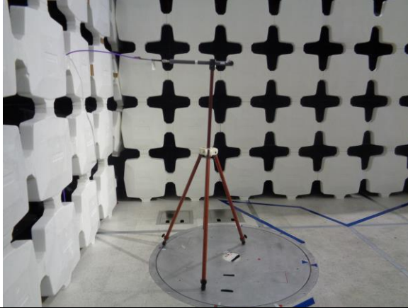
Dipole Antenna Setup
