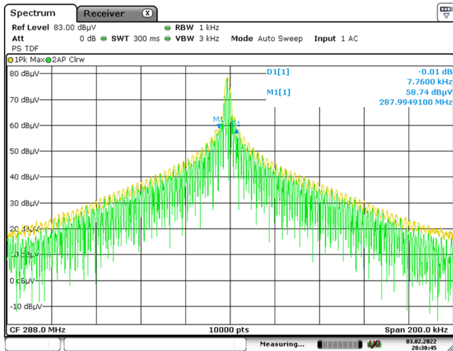
Measuring Occupied Bandwidth at -20dB points20
