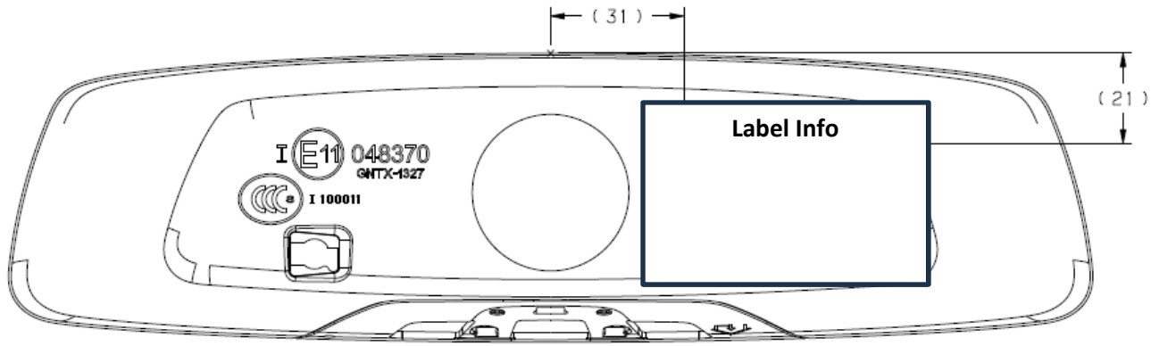
REAR HOUSING VIEW SCALE: 1:1 MOLDED MARKINGS + LASER MARKINGS (340-1328-000) FOR REFERENCE ONLY
