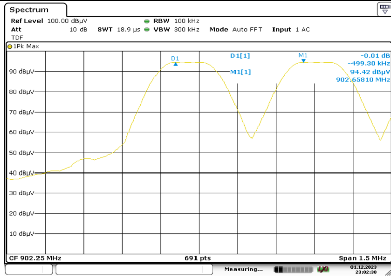
Channel Separation Low Band Measurement Plot
