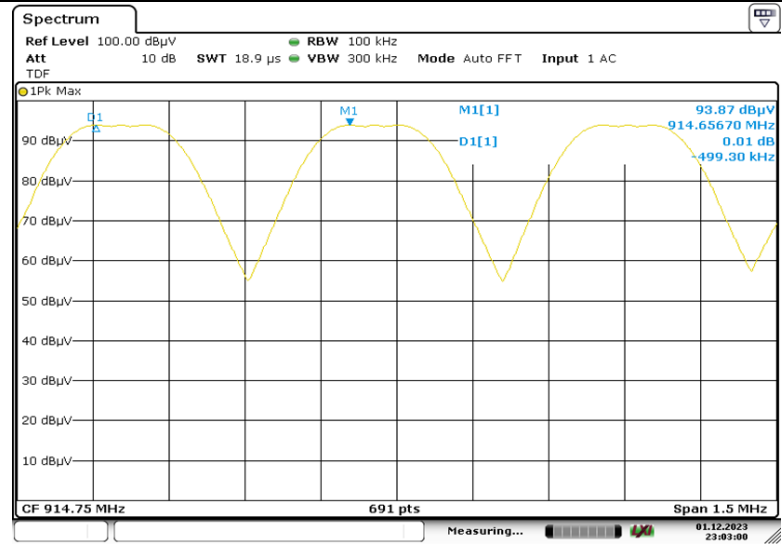
Channel Separation Mid Band Measurement Plot
