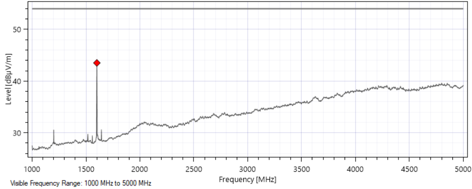
Horizontal Polarization – Flat Orientation - Average
