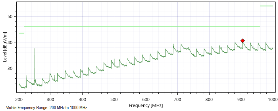
Horizontal Polarization – Flat Orientation
