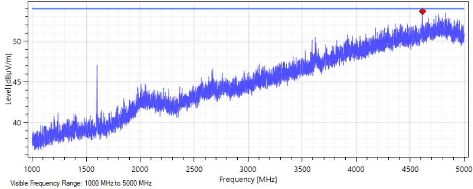
Vertical Polarization – End Orientation – Peak
