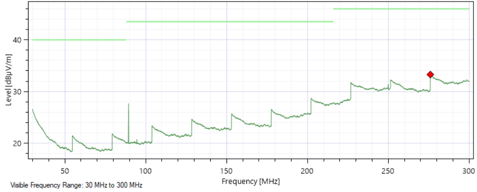
Horizontal Polarization – Side Orientation
