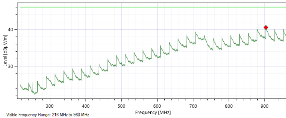
Horizontal Polarization – End Orientation
