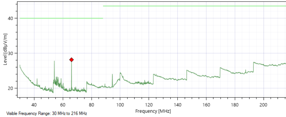
Vertical Polarization – End Orientation
