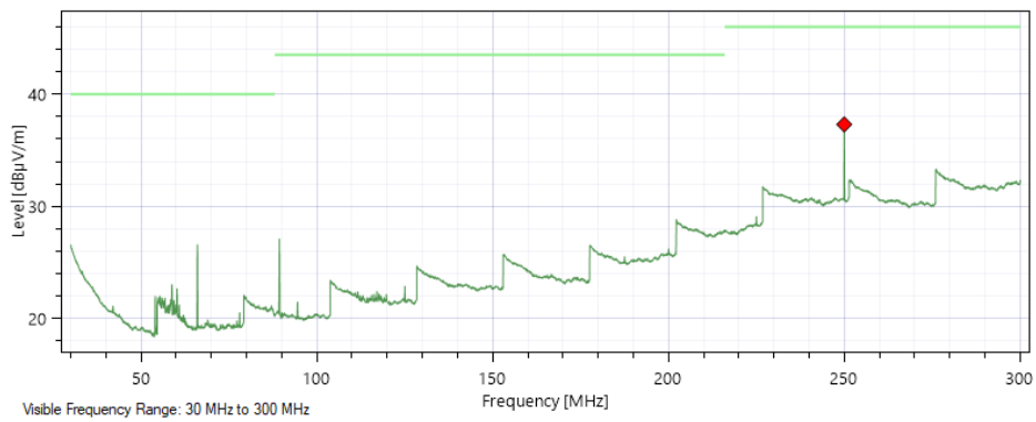
Vertical Polarization – Side Orientation
