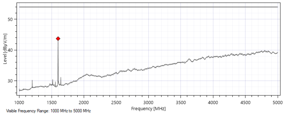
Horizontal Polarization – Side Orientation – Average
