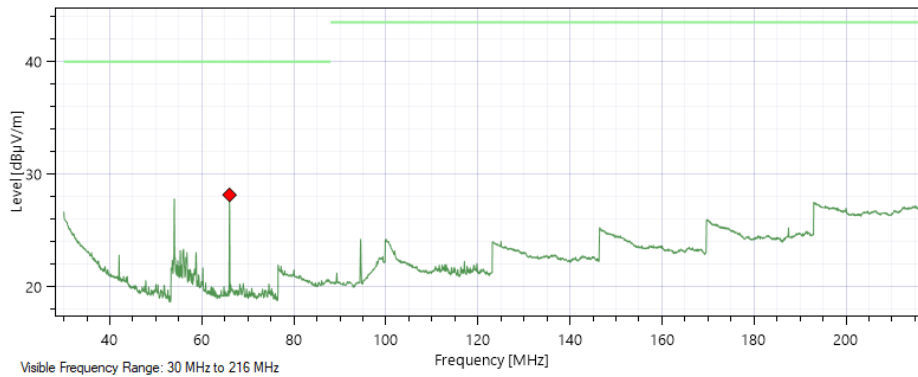
Vertical Polarization – Flat Orientation
