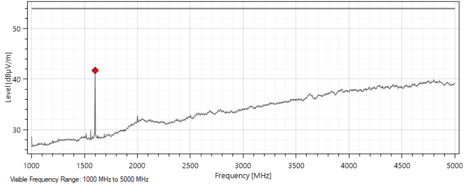
Vertical Polarization – Side Orientation - Average
