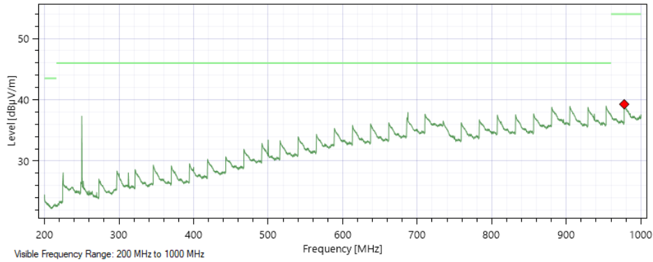
Vertical Polarization – Flat Orientation
