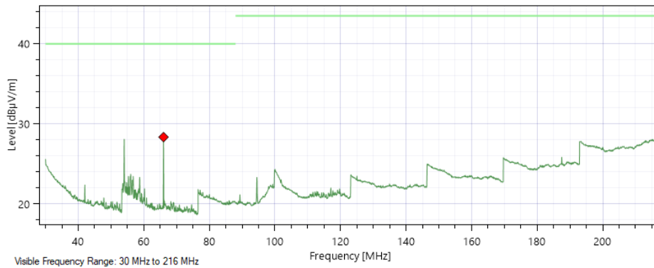
Horizontal Polarization – Flat Orientation
