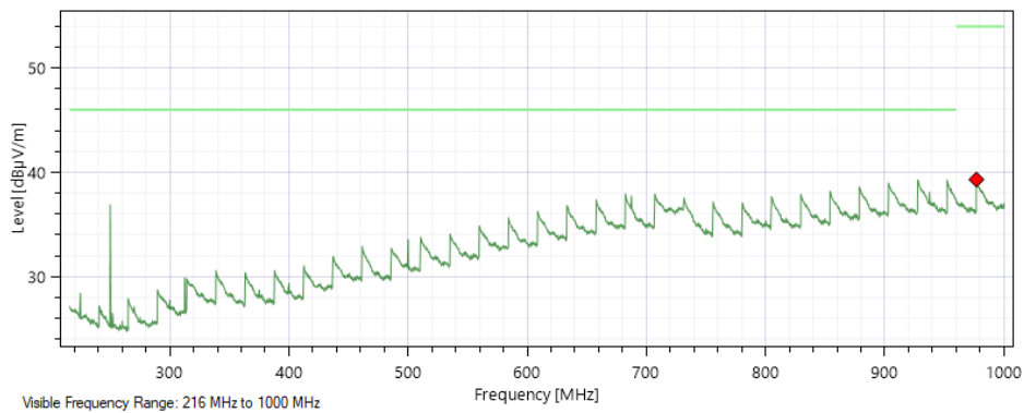
Vertical Polarization – Side Orientation
