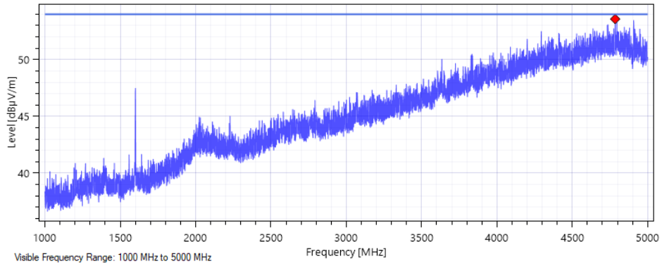
Horizontal Polarization – End Orientation – Peak
