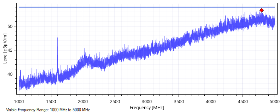
Vertical Polarization – Side Orientation – Peak
