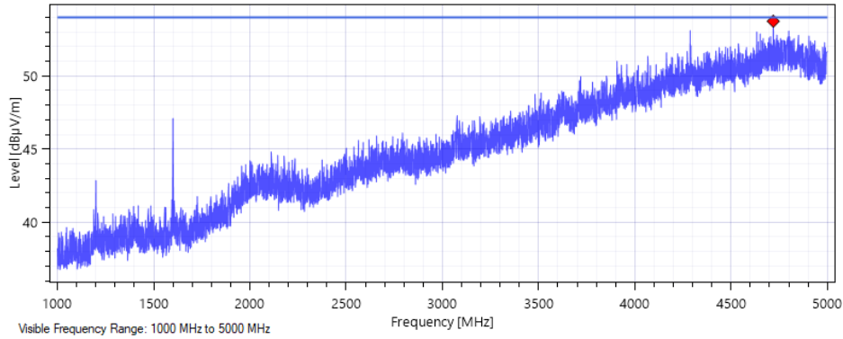
Horizontal Polarization – Side Orientation – Peak
