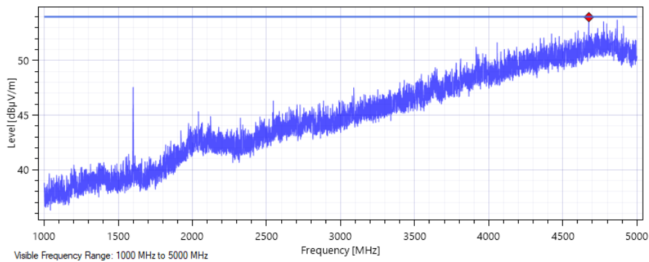
Horizontal Polarization – Flat Orientation – Peak
