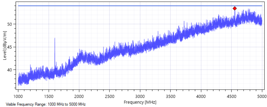
Vertical Polarization – Flat Orientation – Peak
