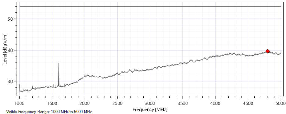
Vertical Polarization – Flat Orientation - Average
