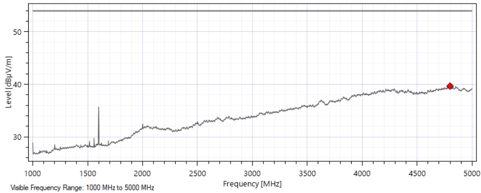
Vertical Polarization – End Orientation - Average
