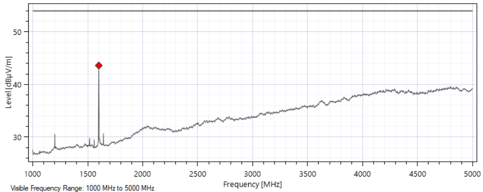
Horizontal Polarization – End Orientation - Average
