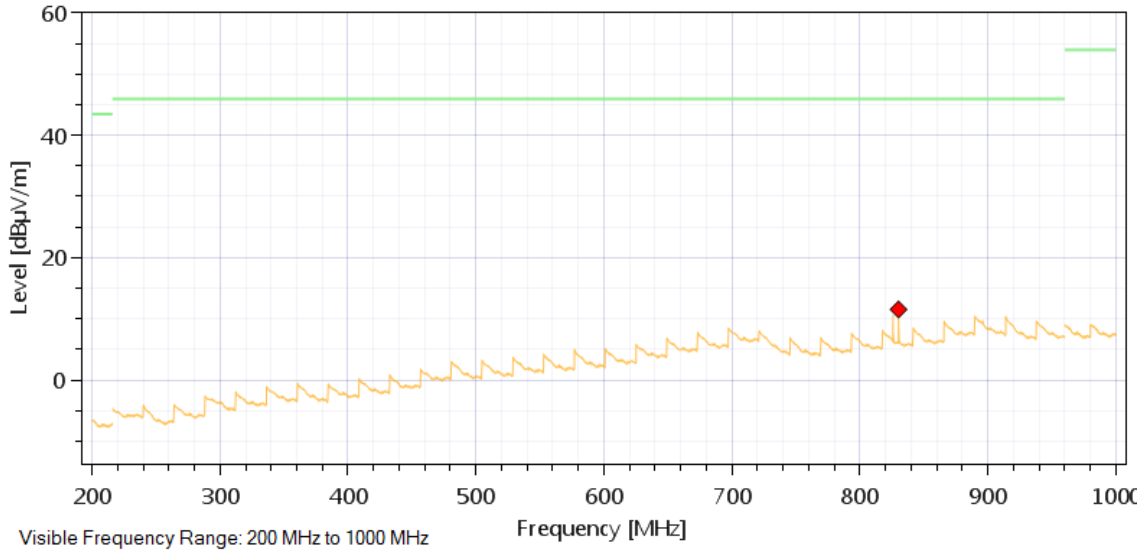
Horizontal Polarization – End
