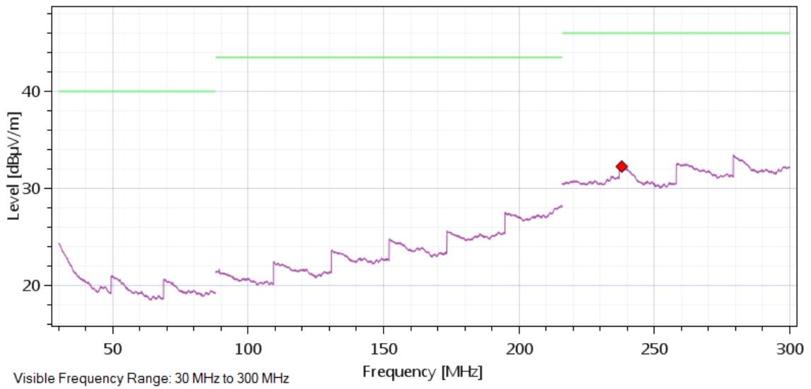
Vertical Polarization - End
