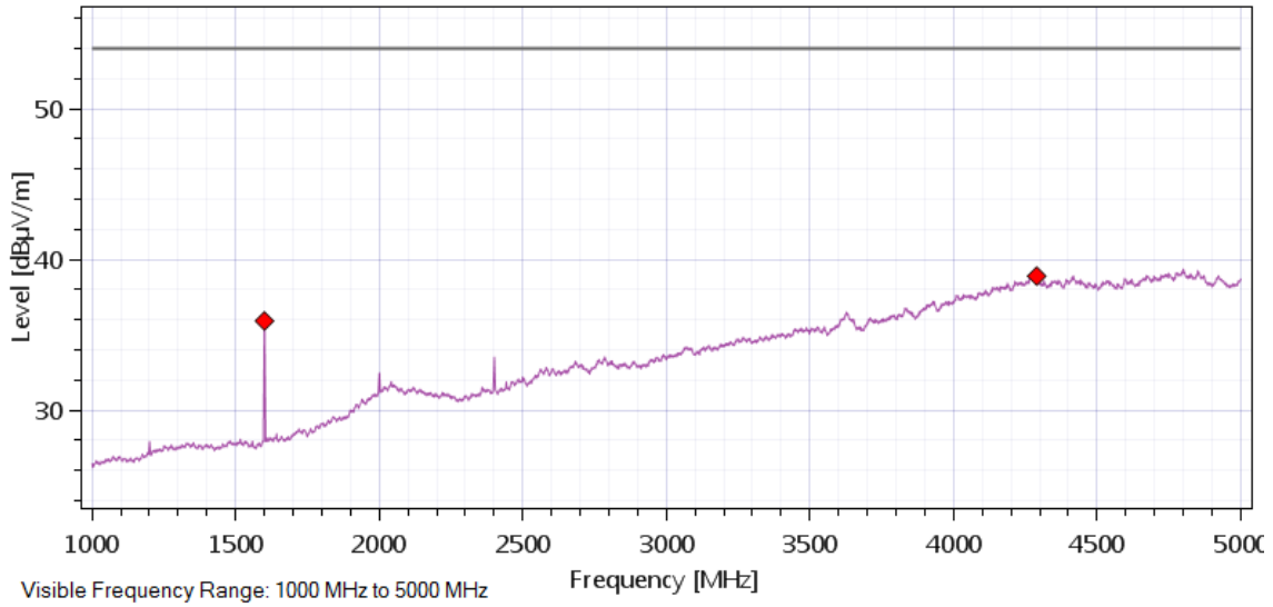
Vertical Polarization – Side
