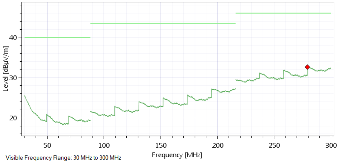
Horizontal Polarization - Side
