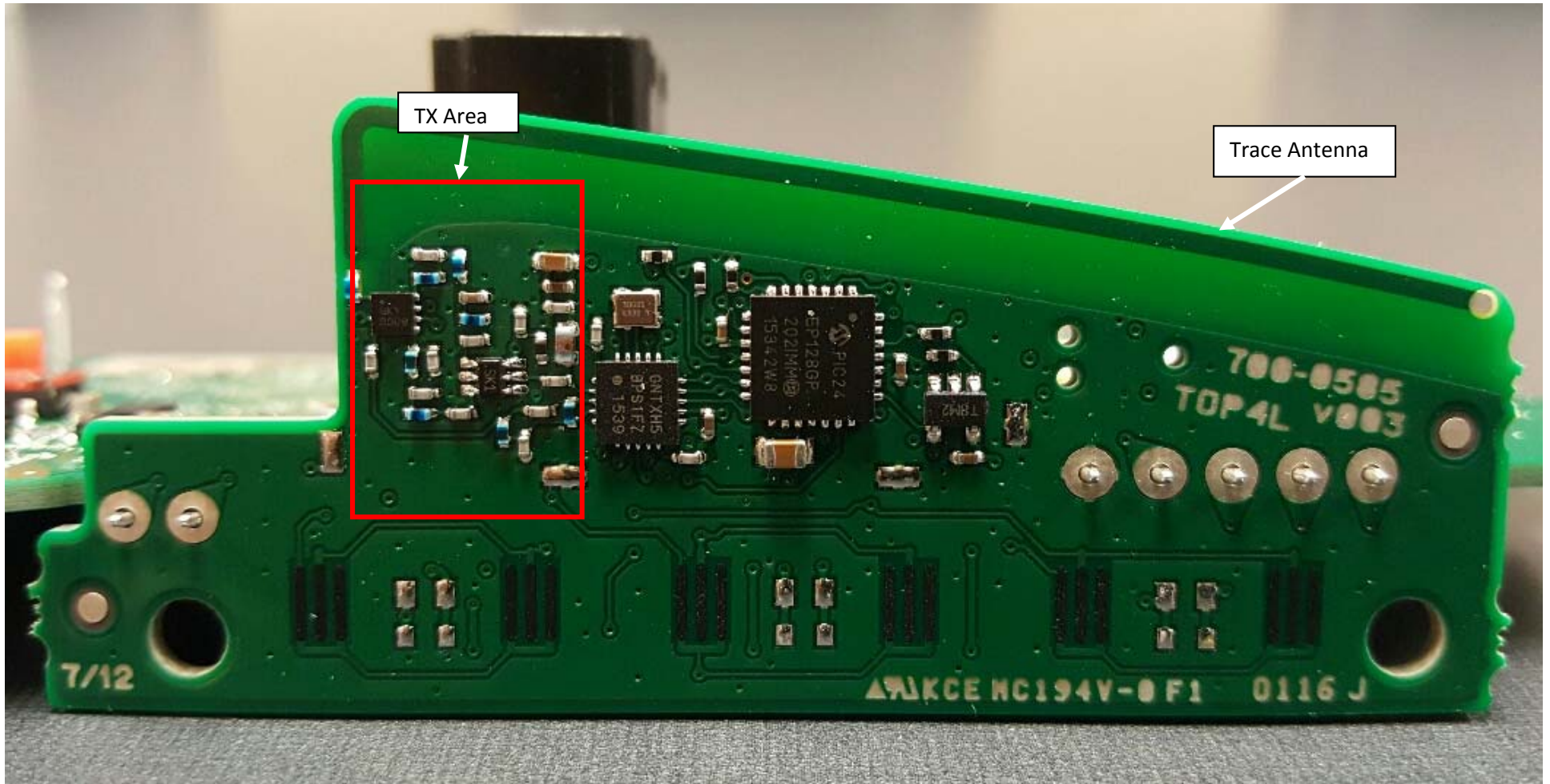
700-0585 – Transmitter Board
