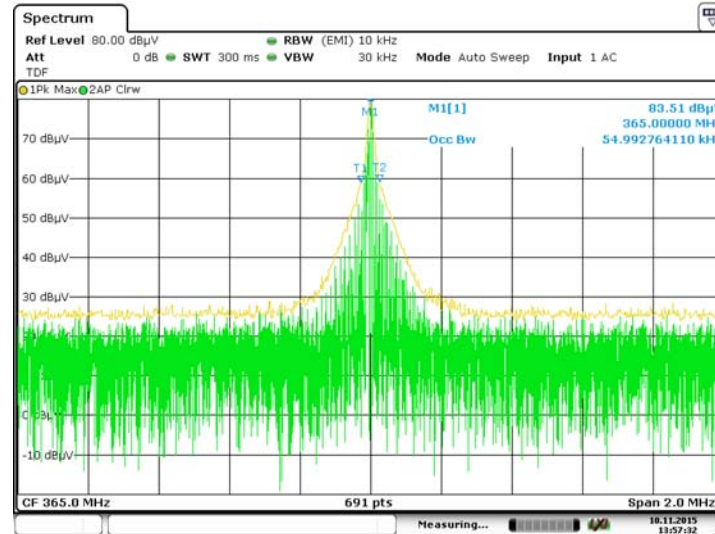
Measuring Occupied Bandwidth at –20dB – 365MHz
