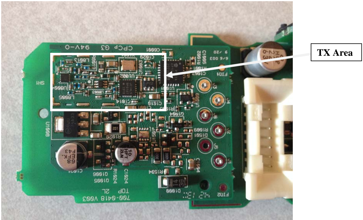
Close-up of Homelink RF Section - Front
