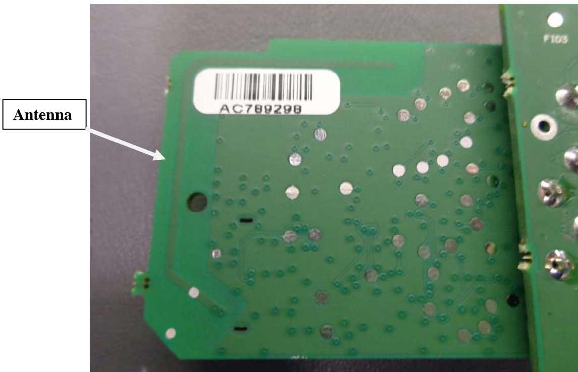
Close-up of Homelink RF Section - Front
