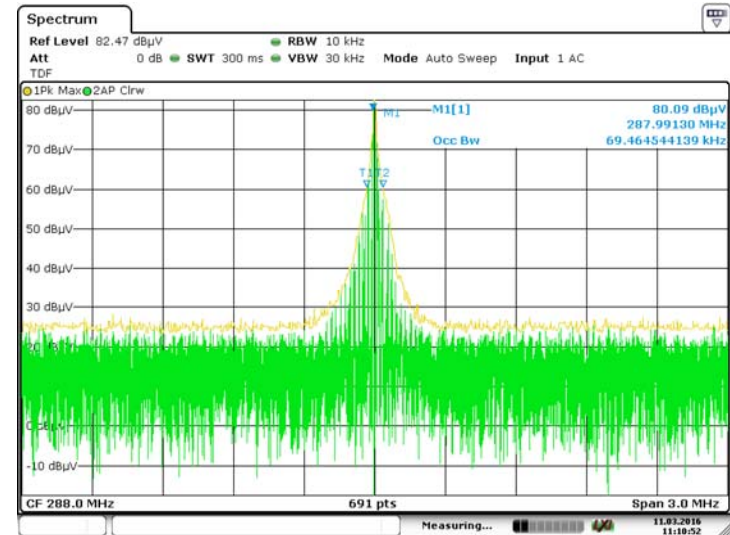
Measuring Occupied Bandwidth at -20dB – 288MHz
