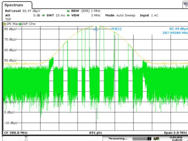
Measuring Peak Reference Level – 288MHz
