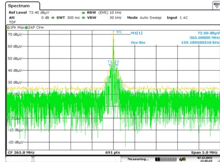
Measuring Occupied Bandwidth at -20dB: 365MHz
