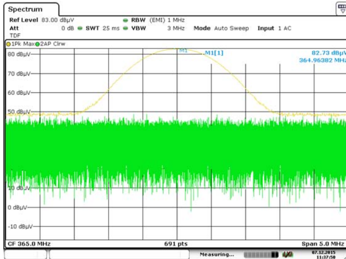
Measuring Peak Reference Level: 365MHz
