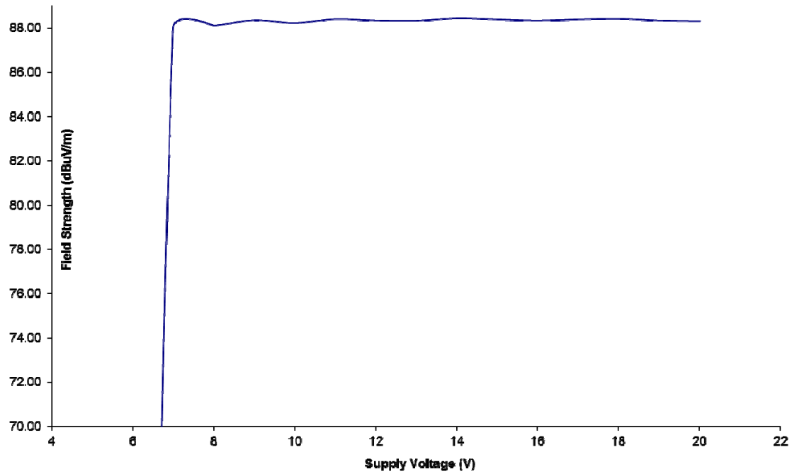
Output Field Strength vs. Supply Voltage
