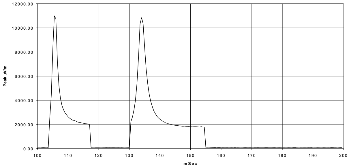
Coarse Tune Pulses, 310MHz fundamental Linear Scale
