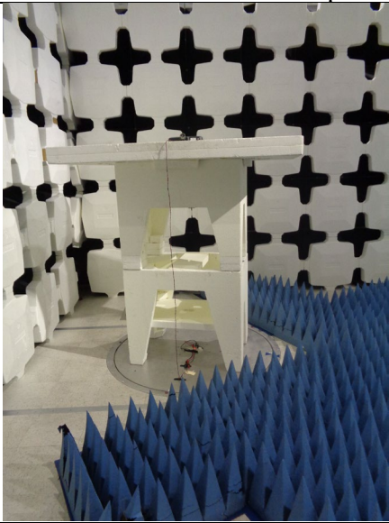
LPA (200-1000MHz) Setup Overview
