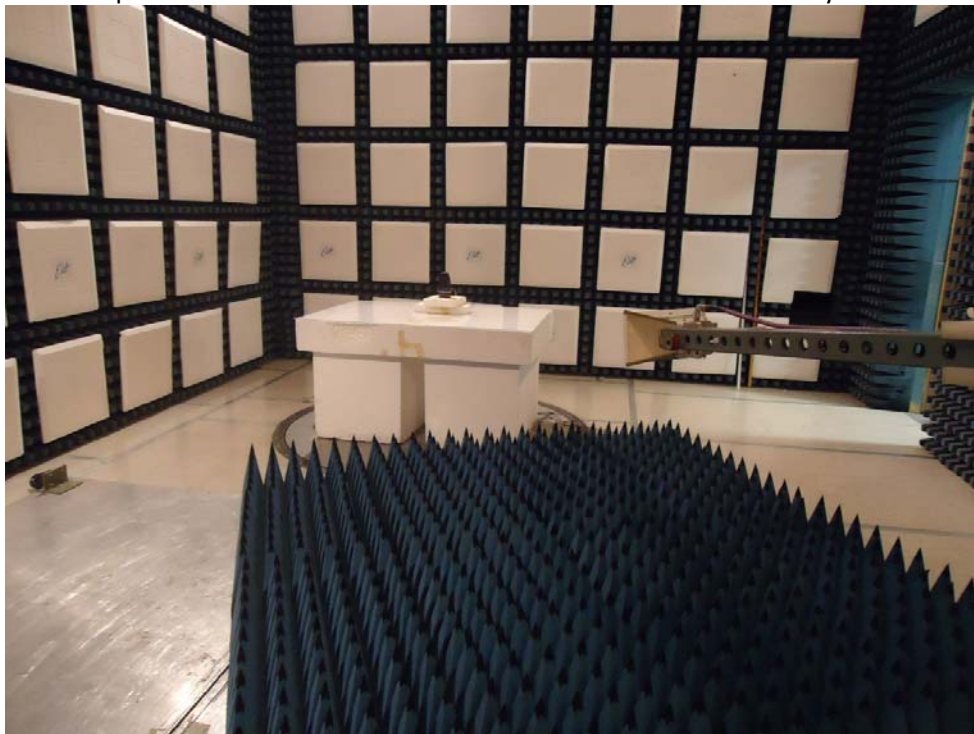
Test Setup for Radiated Emissions above 1000MHz Vertical Polarity
