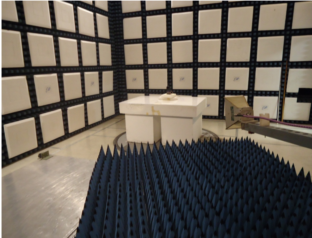
Test Setup for Radiated Emissions above 1000MHz Horizontal Polarity
