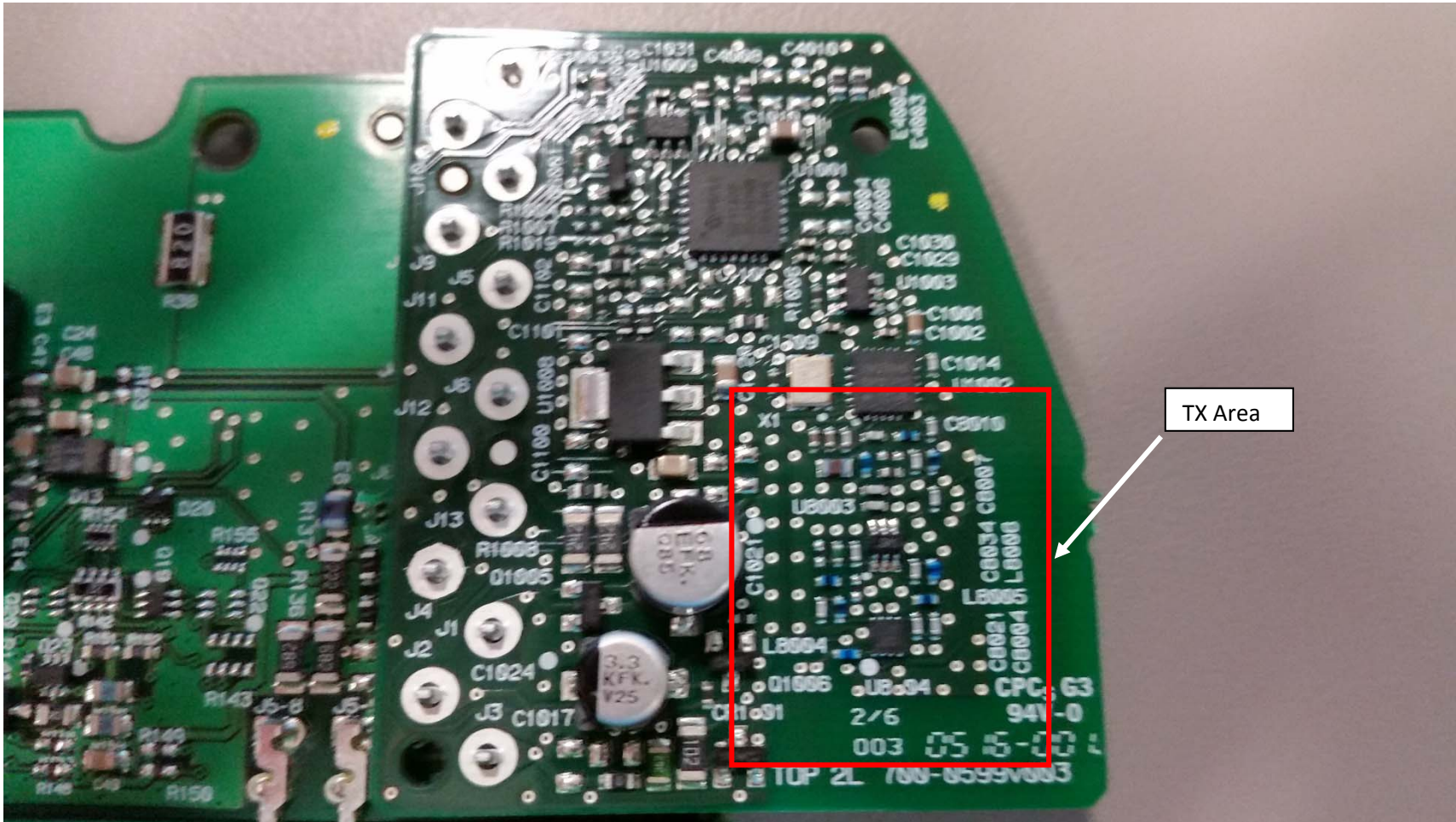
700-0599 – Transmitter Board
