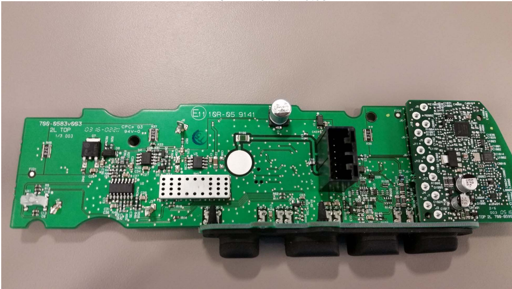
700-0583 – Mother Board
