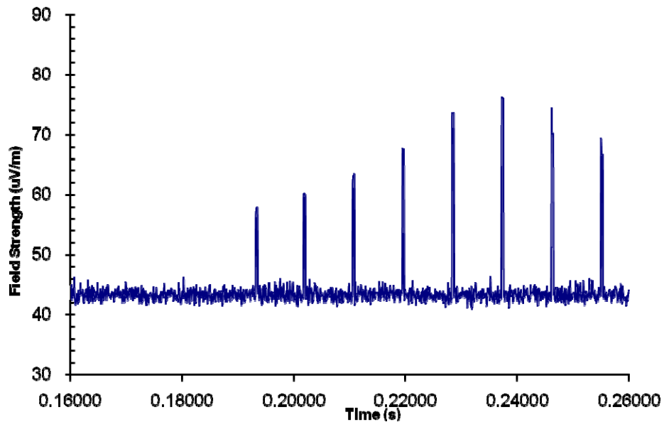
288 MHz, 30% Duty Cycle Tuning Pulse
