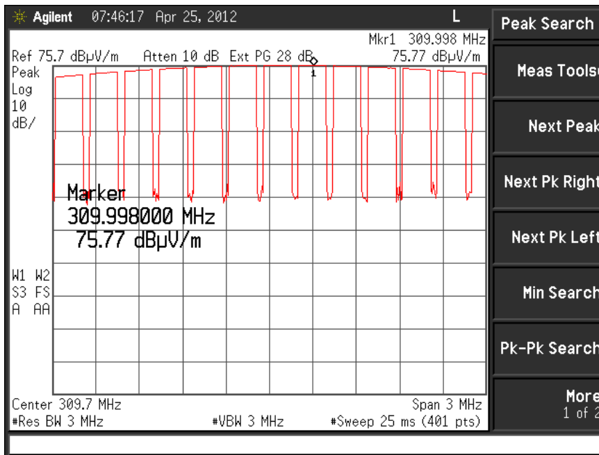
Measuring Peak Reference Level
