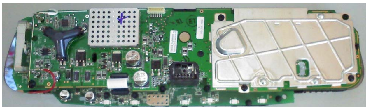
705-0430 Motherboard and Daughter Card Assembly
