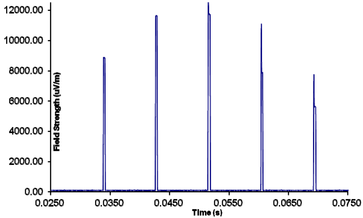
310 MHz, 30 % Duty Cycle Tuning Pulse
