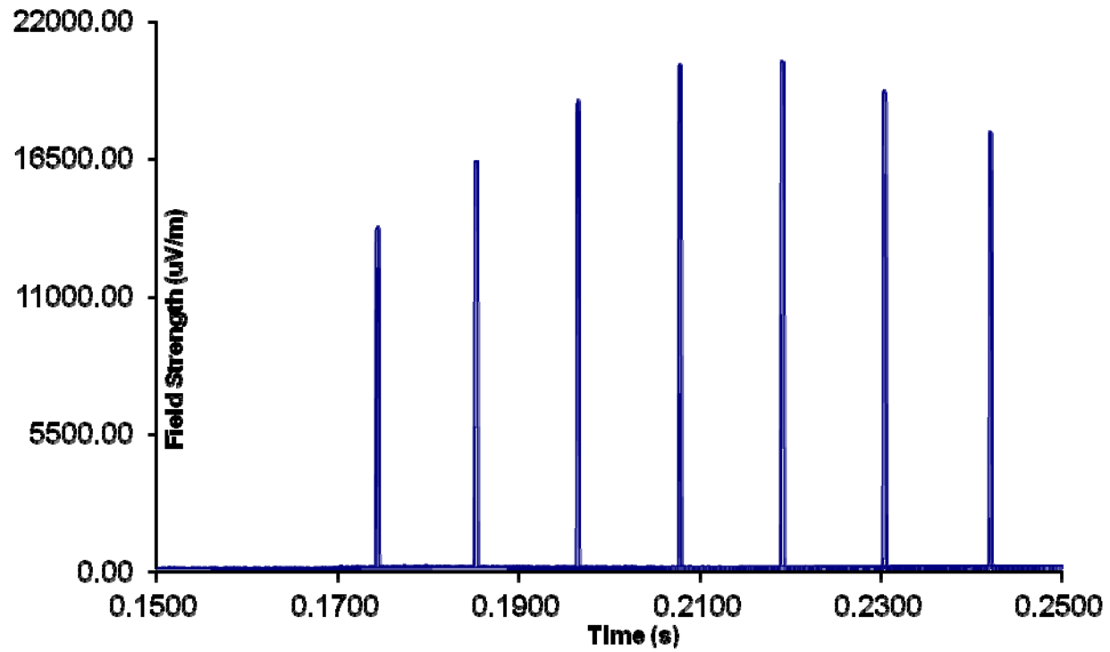
433 MHz, 30 % Duty Cycle Tuning Pulse ( 100ms window )
