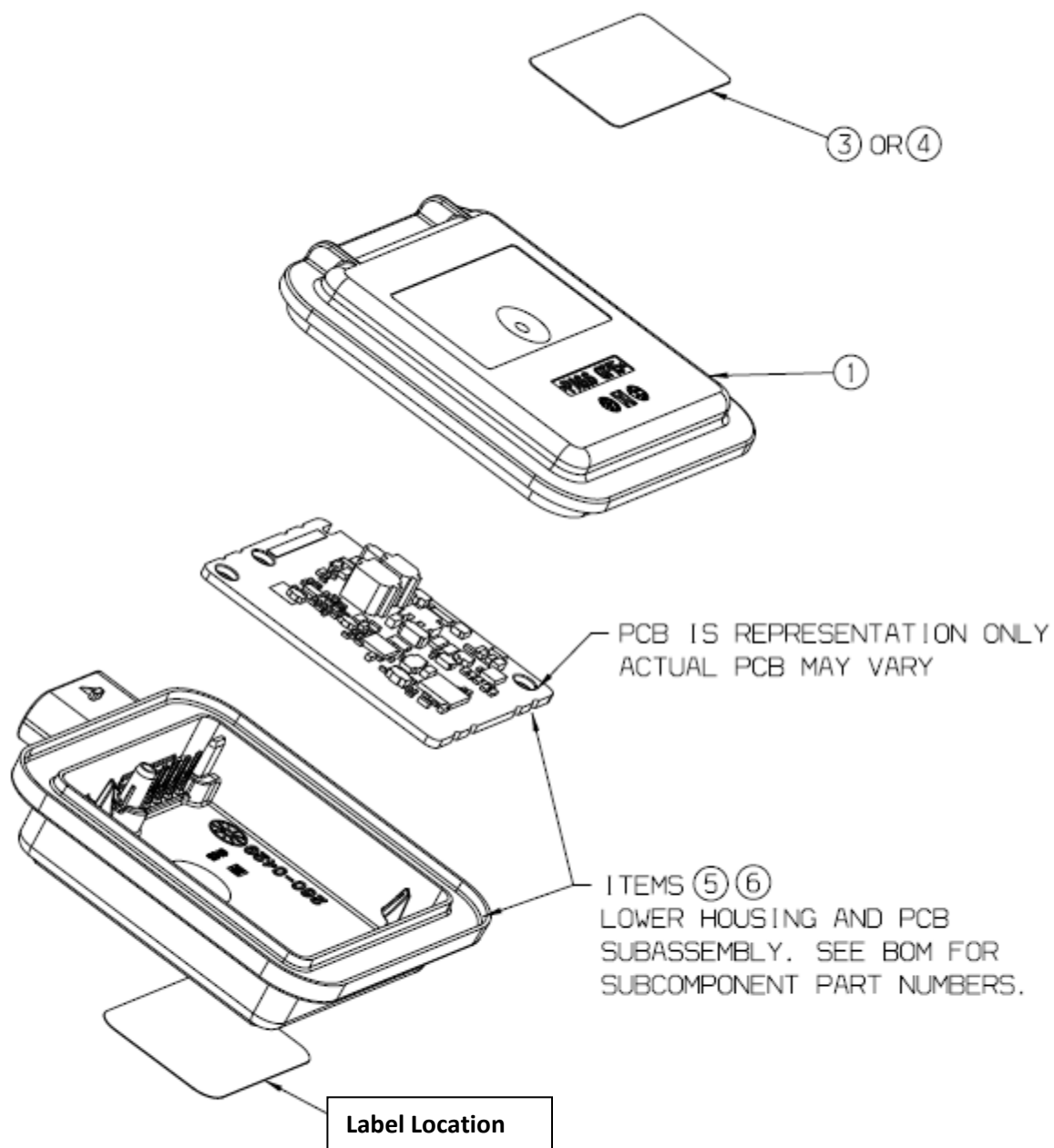
EXPLODED VIEW
