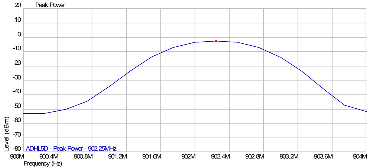
ADHL5D - Peak Power - 902.25MHz Peaks
