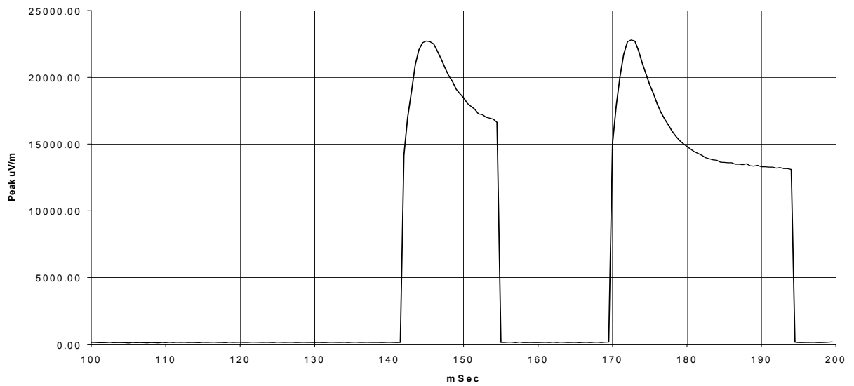
Coarse Tune Pulses, 418MHz fundamental Linear Scale
