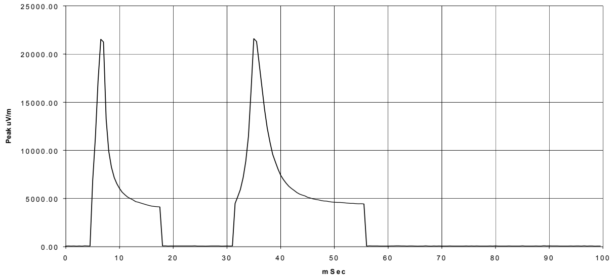
Coarse Tune Pulses, 310MHz fundamental Linear Scale
