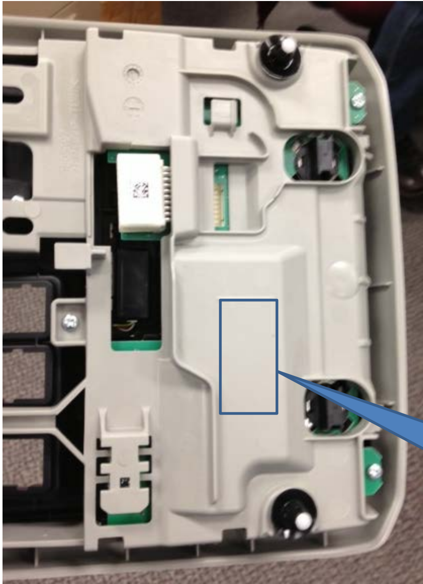
Homelink FCC Label Placement Location
