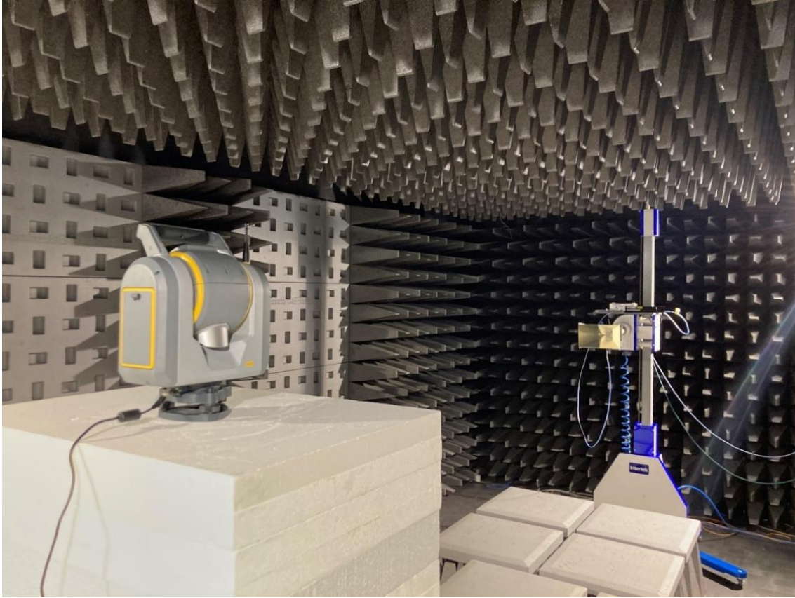
Photo of the test set-up for radiated emission above 1 GHz
