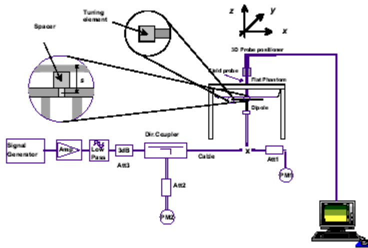
System Check Set-up
