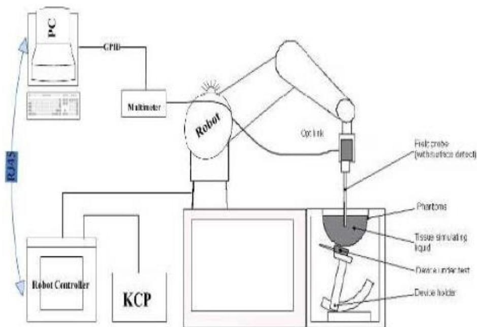
KUKA SAR Test System Configuration
