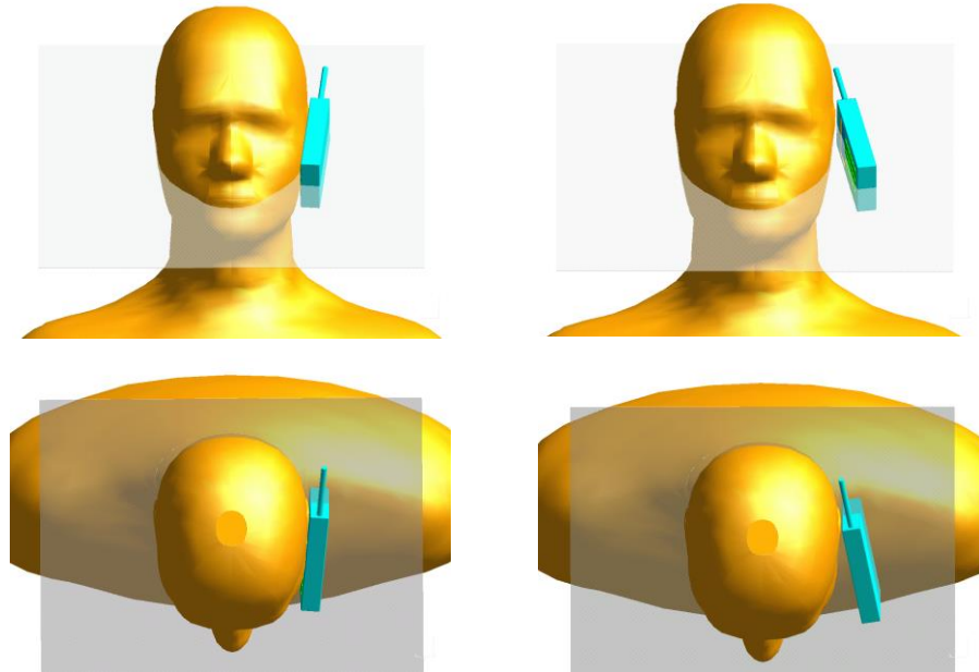
Fig1:Cheek and Tilt positions requested by CENELEC and IEEE
