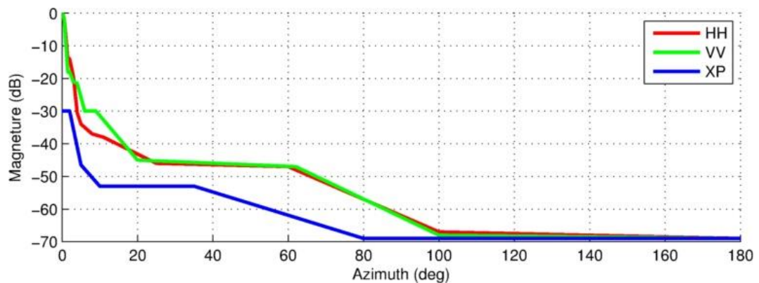
0.6m 27.50-29.60 GHz RADIATION PATTERN ENVELOPE
