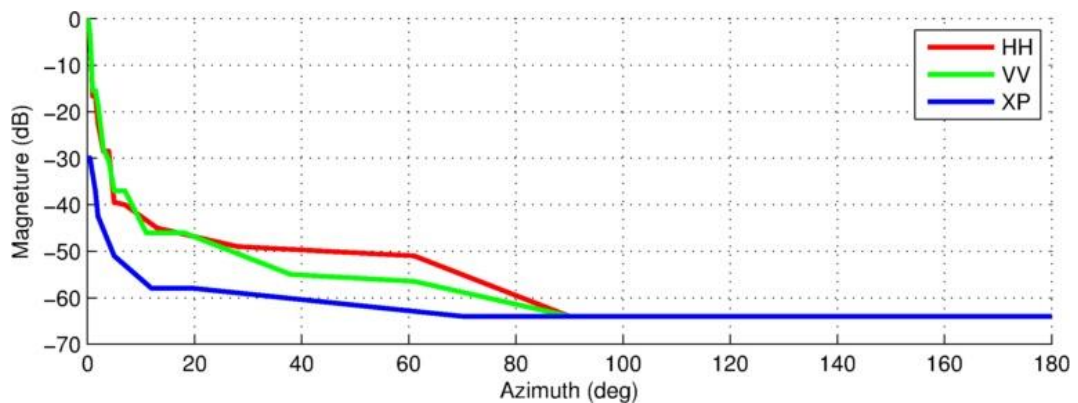
0.6m 40.50-43.50 GHz RADIATION PATTERN ENVELOPE
