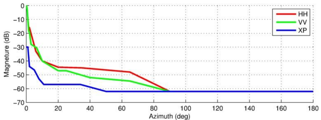
0.6m 31.80-33.40 GHz RADIATION PATTERN ENVELOPE
