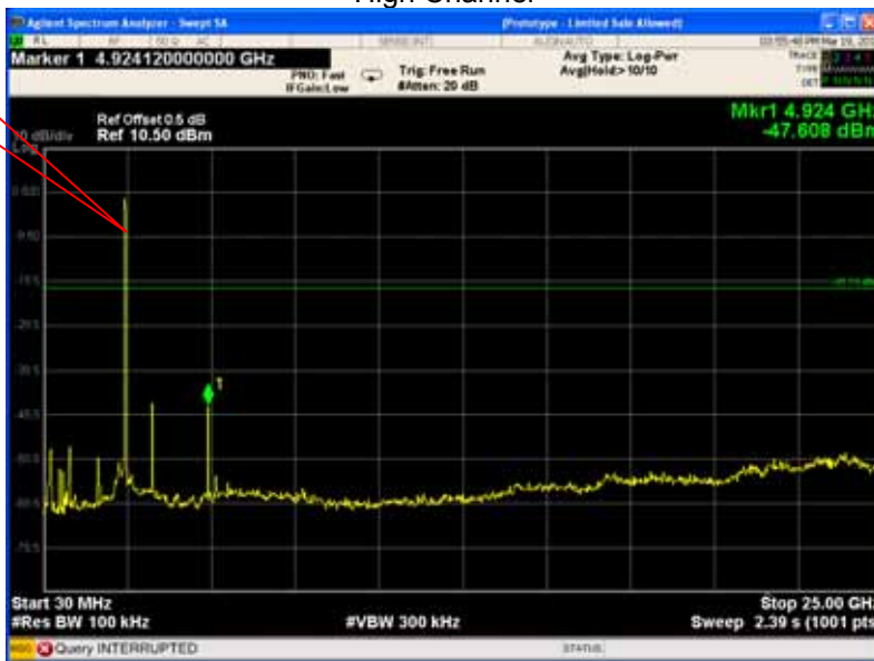
High Channel
