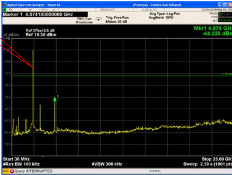
Middle Channel
