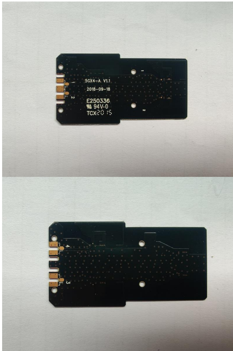
Size specifications: length 50.1mm, width 26.6mm, thickness 0.4mm
