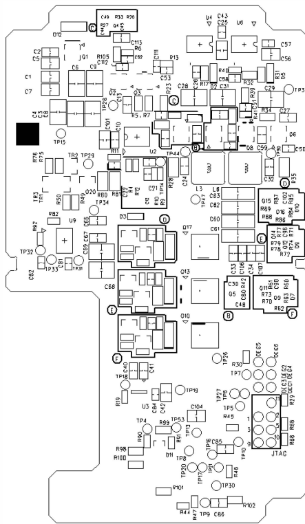
SILKSCREEN BOTTOM
