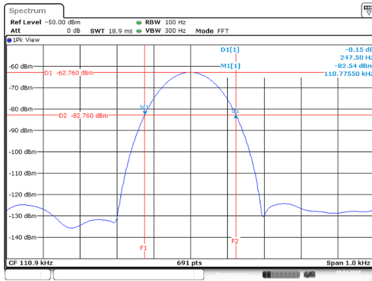
Emission Bandwidth Plot 20dB Bandwidth (110.90kHz)
