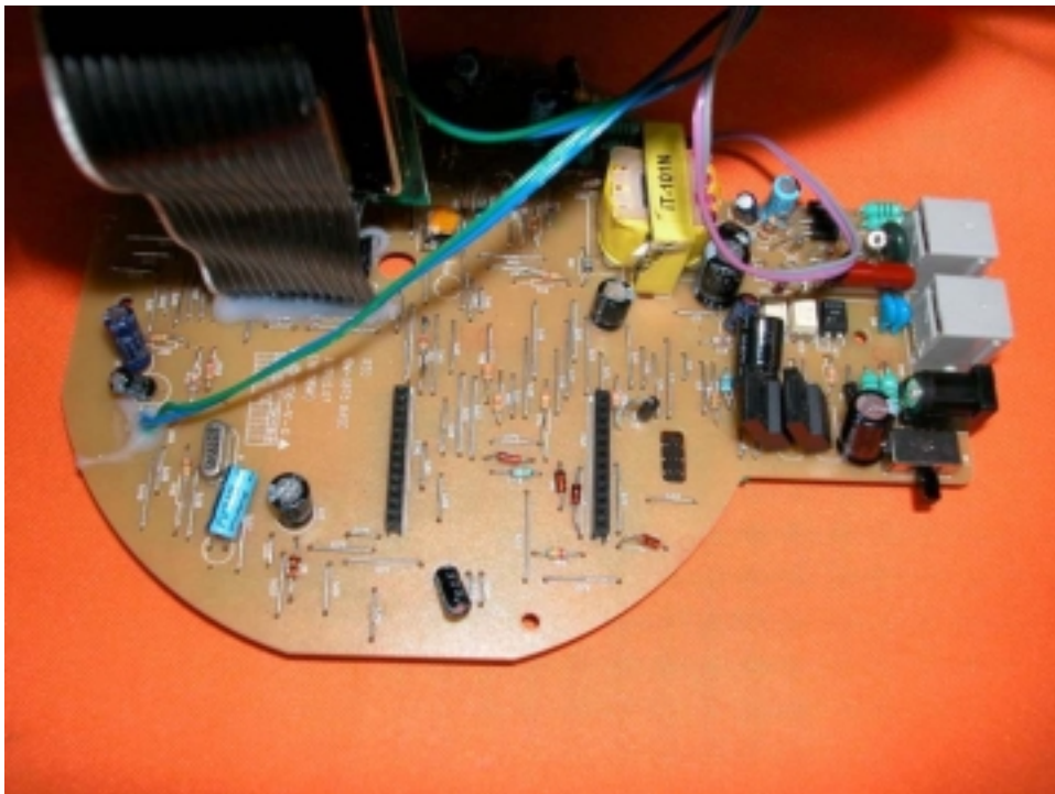
Base Main PCB solder side (View 3)
