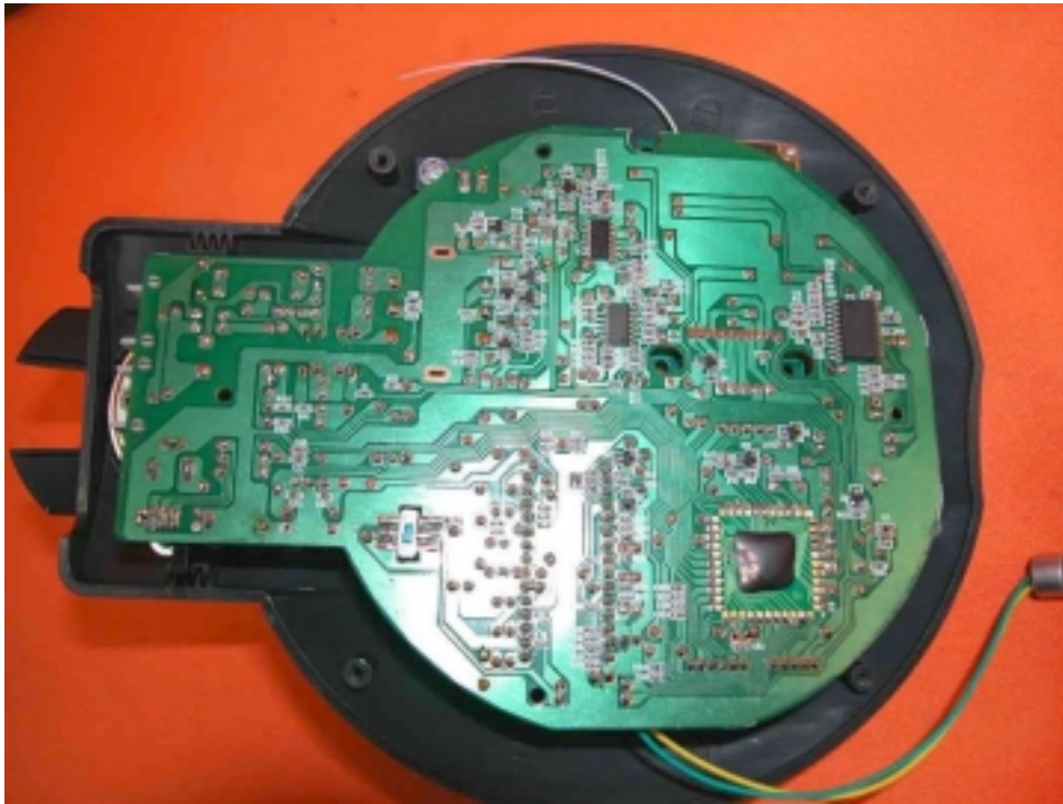
Speakerphone PCB keypad side
