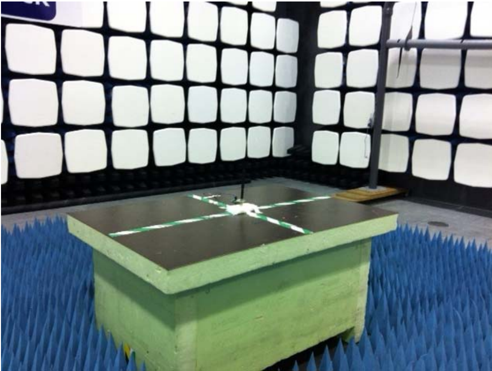
Radiated spurious emission 1-10 GHz
