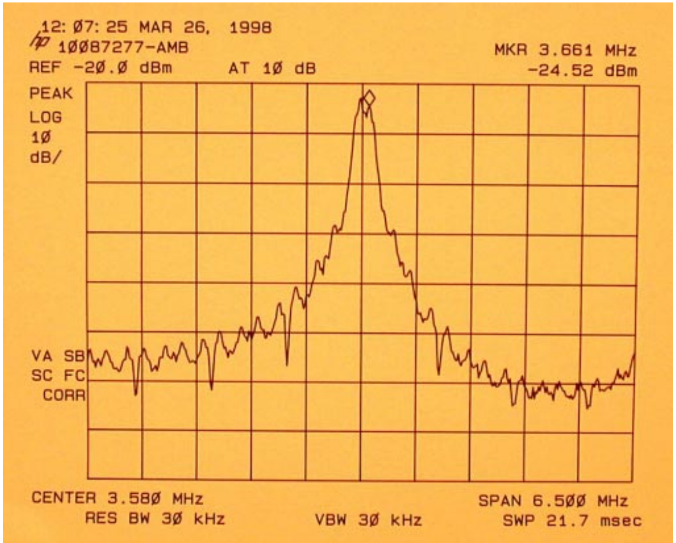
Plot 3 - Carrier bandwidth TranX 260
