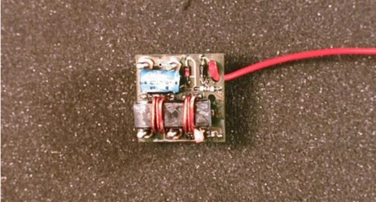
Internal photo TranX 120 (top)
