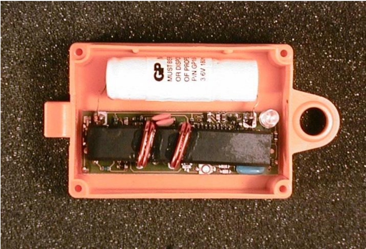
Internal photo TranX 160 (top)
