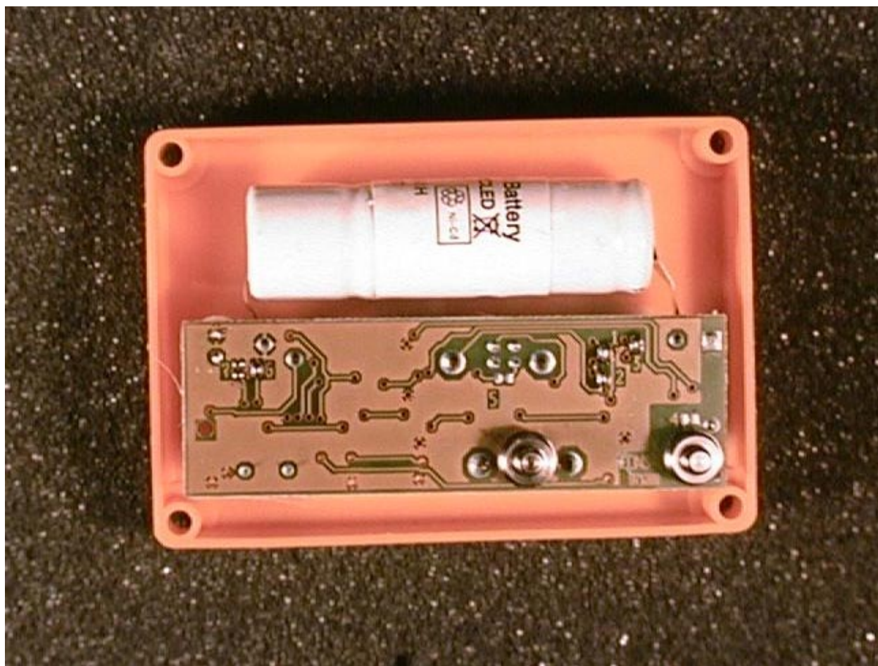
Internal photo TranX 160 (bottom)
