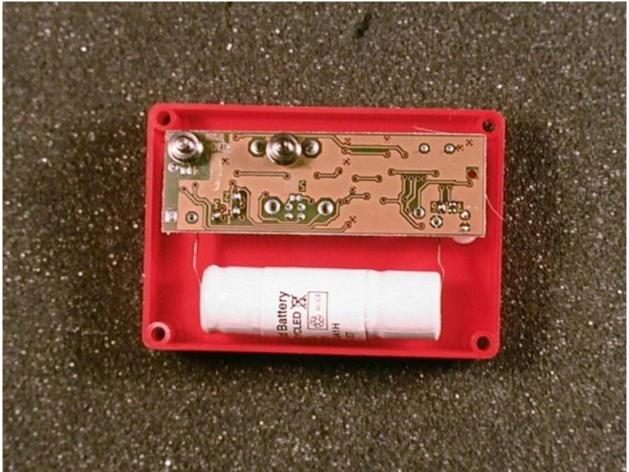
Internal photo TranX 260 (bottom)
