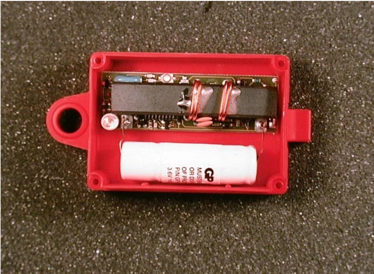
Internal photo TranX 260 (top)
