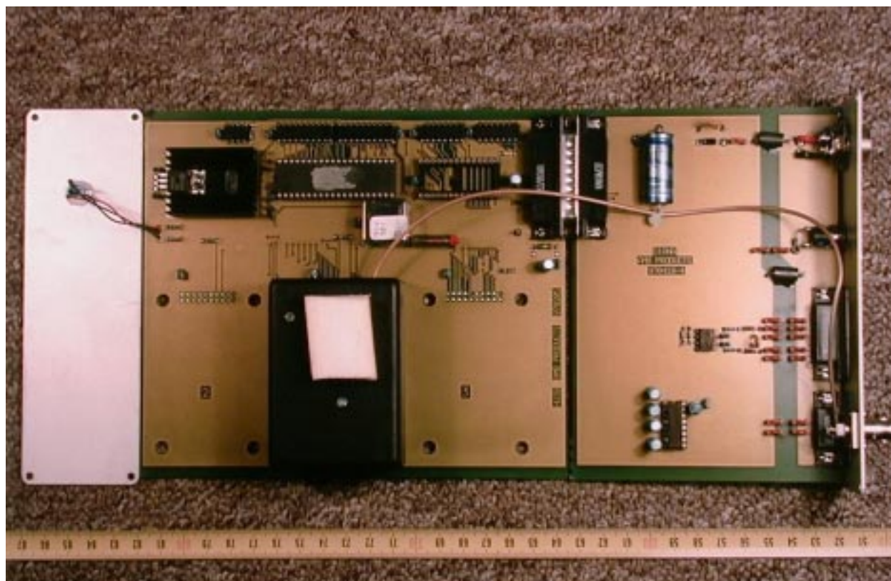
Internal photo TranX decoder (top)
