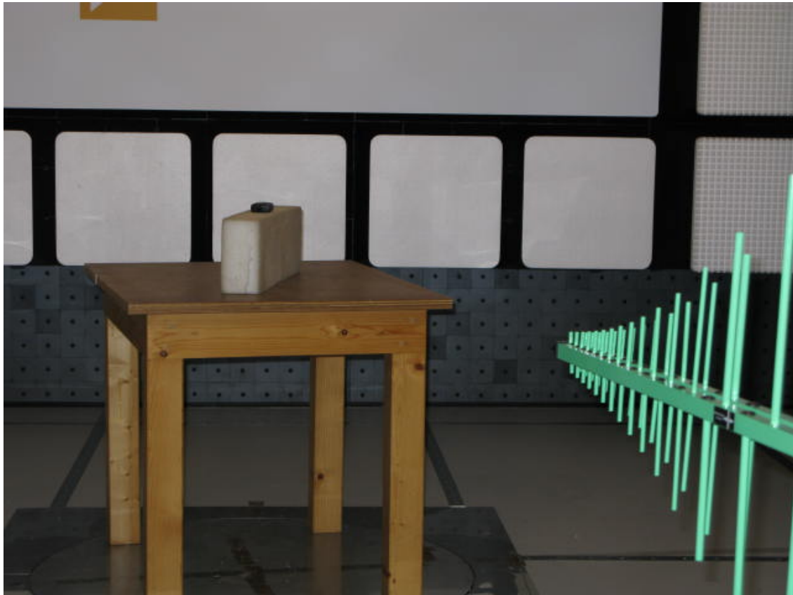
Photograph 1: Test setup field strength measurements ( \geq 30 MHz)
