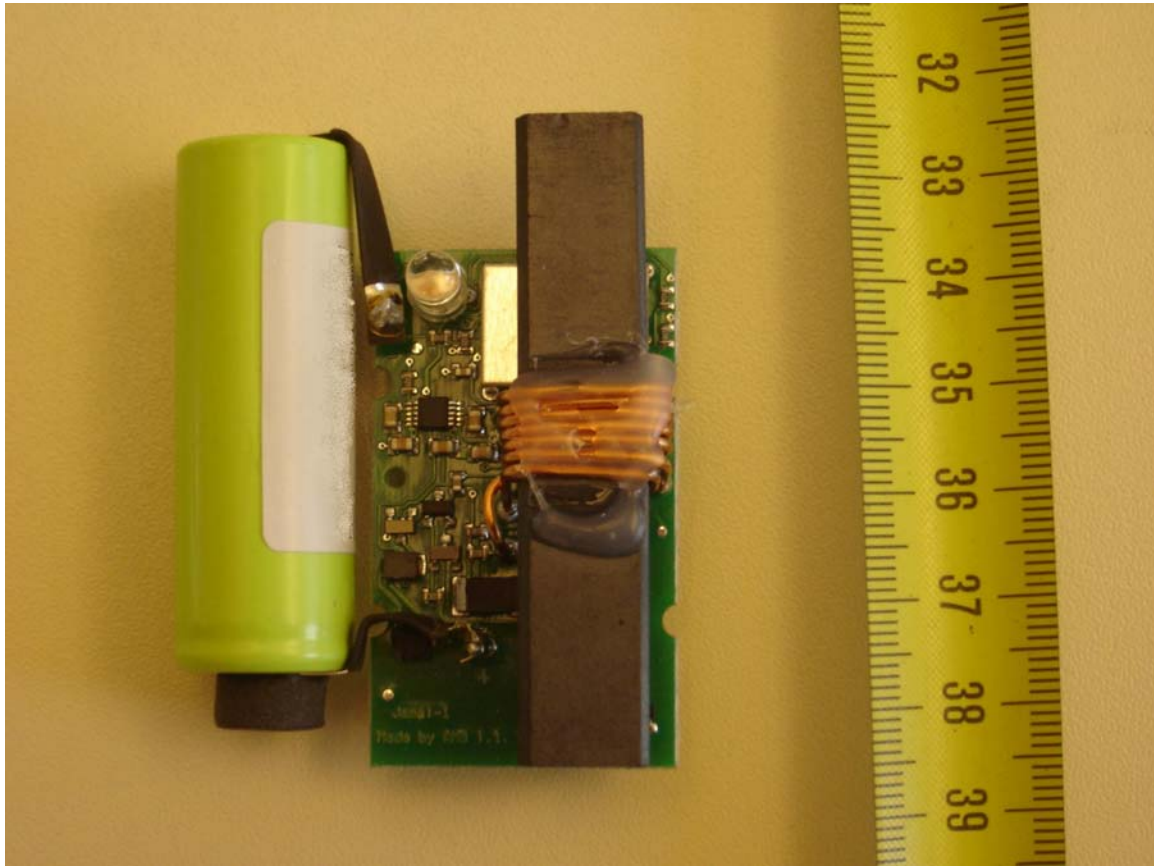
Photograph 1: TnetX Pro Communicator Lite, PCB top view
