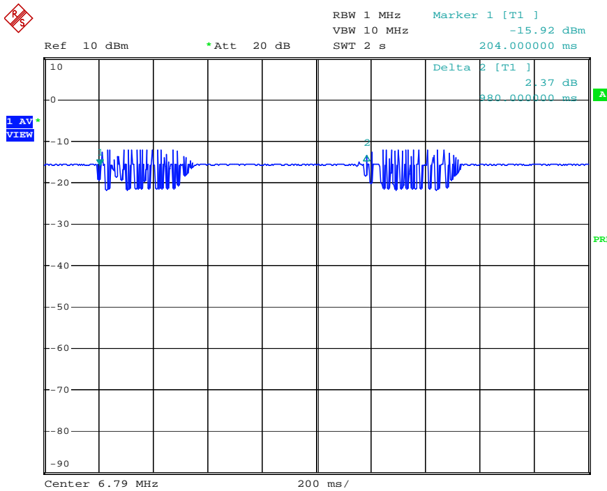
Plot 4: Emissions in Zero-span over 2 seconds period, average detector
