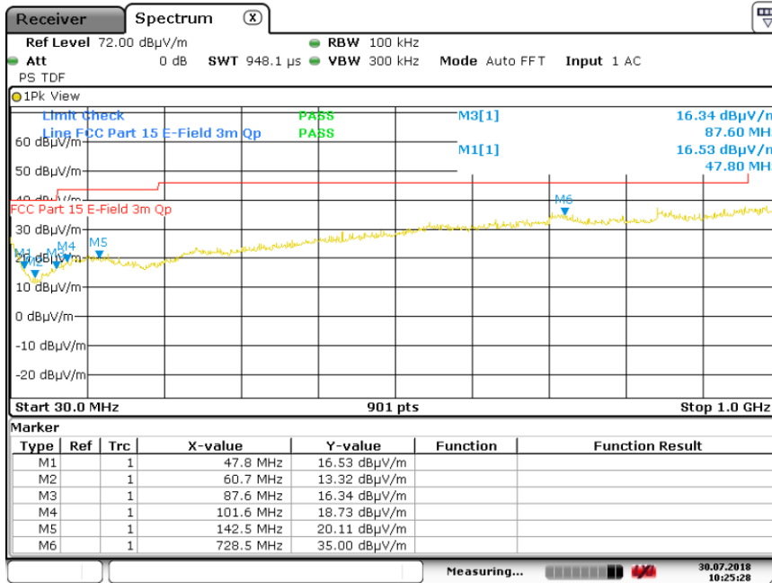
Plot 4: radiated emissions (peak values shown) of the EUT (vertical), Antenna horizontal
