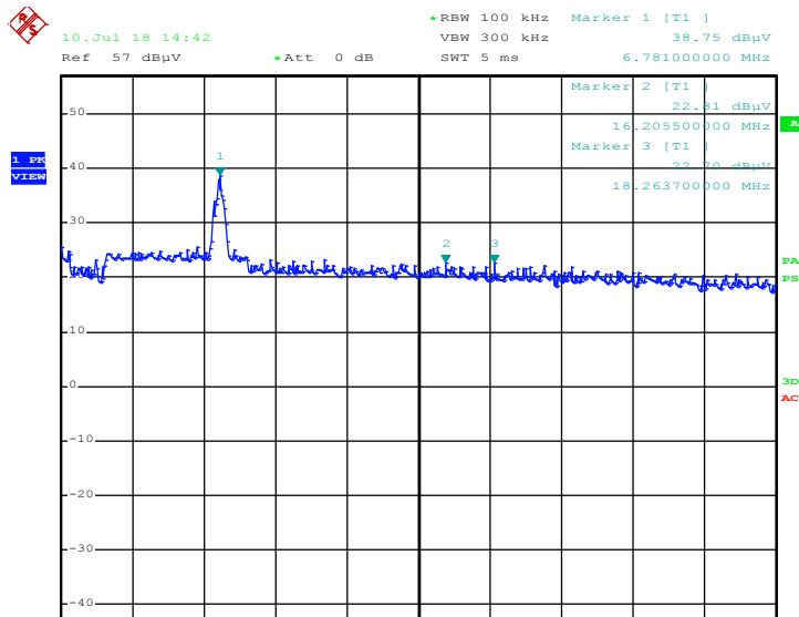
Plot 1: the emissions, EUT Vertical, Peak values shown
