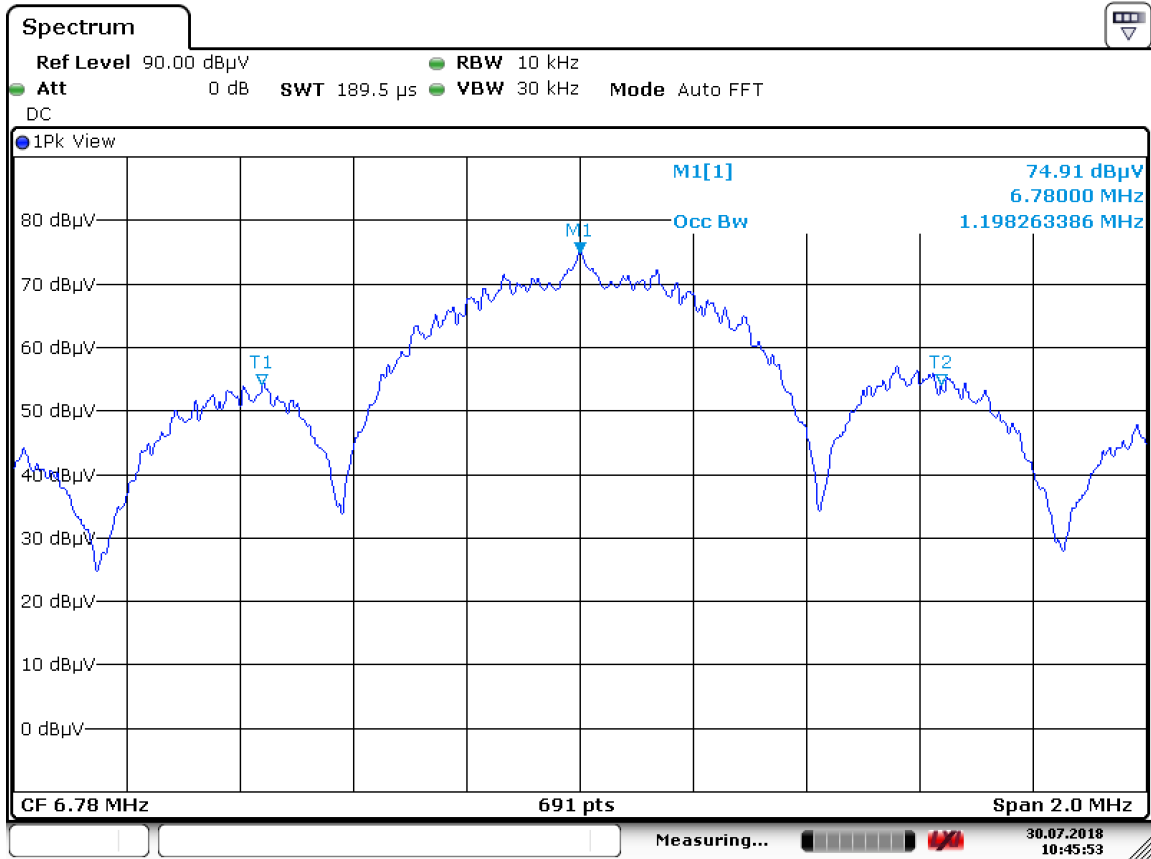
Plot 7: 20 dB bandwidth of the fundamental, actual bandwidth is kHz as measured on a spectrum analyzer
