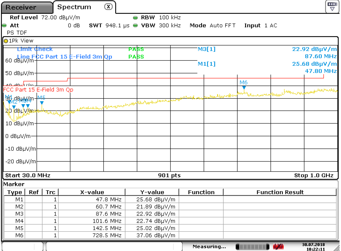
Plot 5: radiated emissions (peak values shown of the EUT (vertical), Antenna vertical)
