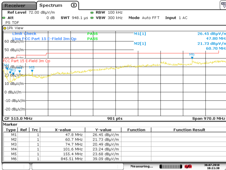
Plot 3: radiated emissions of the EUT (Horizontal), (peak values shown), Antenna horizontal
