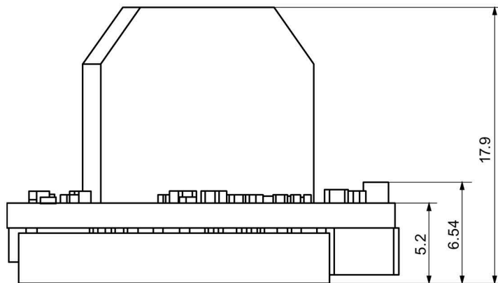
Figure 2-1 Dimension drawing SIMATIC RTLS PCB OEM AC - All dimensions specified in millimeters
