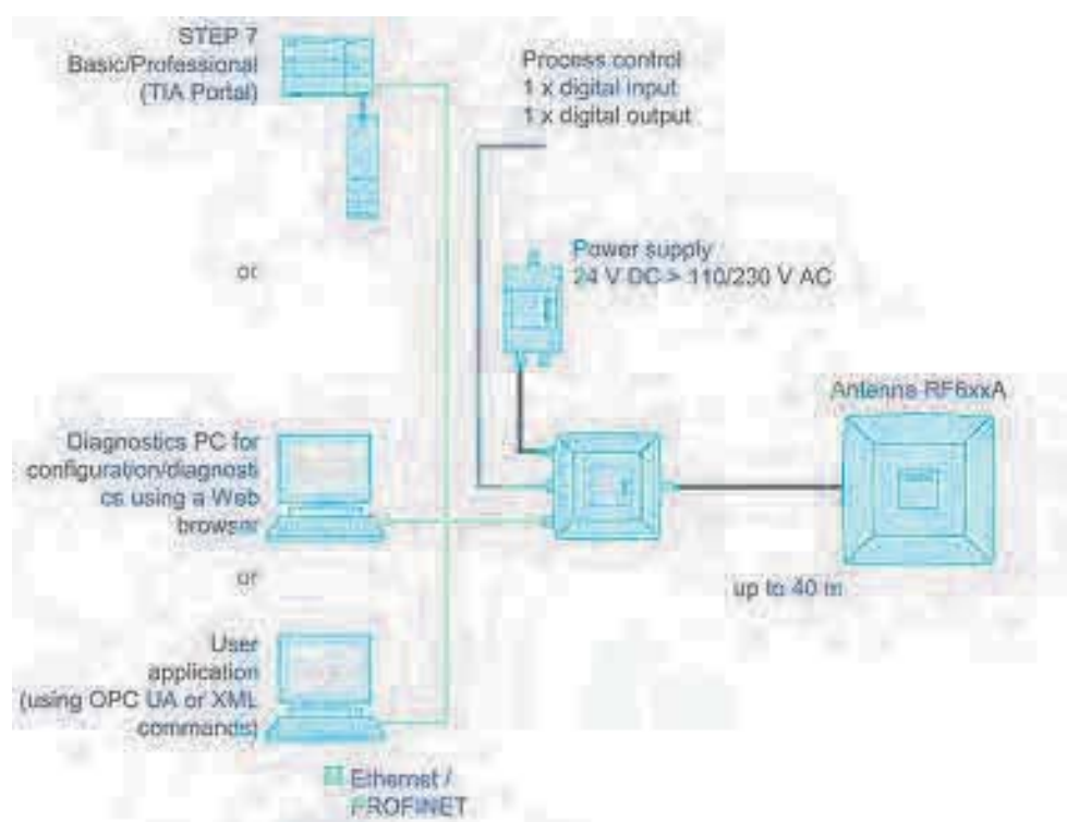
Figure 5-13 Overview: Configuration of RF615R readers
