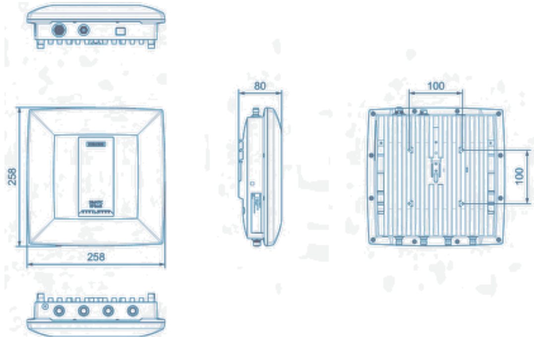
Figure 5-23 Dimension drawing RF650R
