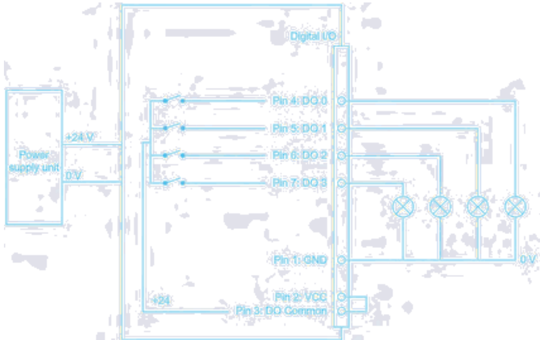
Figure 5-28 Circuit example 4: Digital outputs
