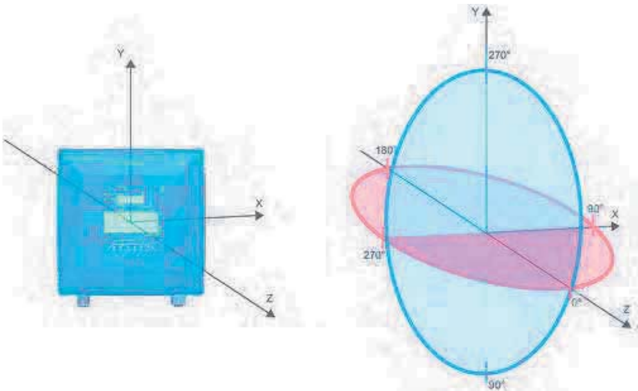
Figure 5-3 Reference system
