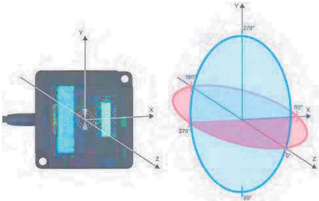
Figure 6-5 Reference system
