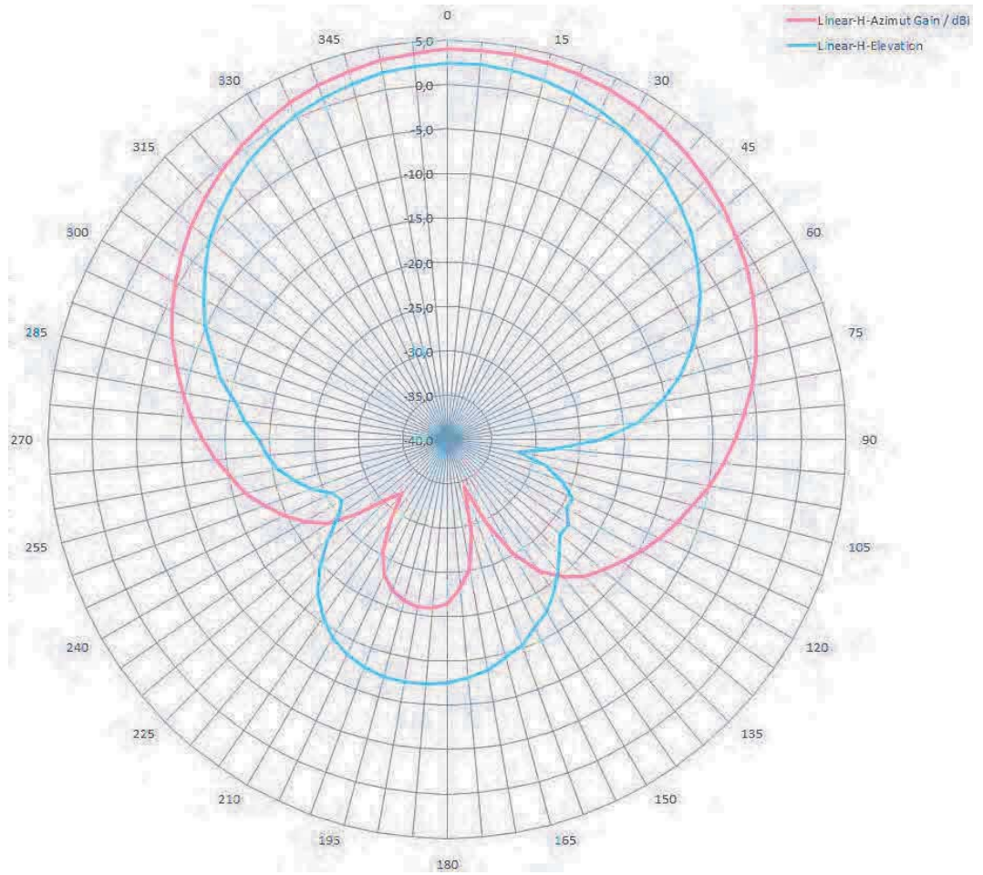
Figure 5-46 Elevation section
