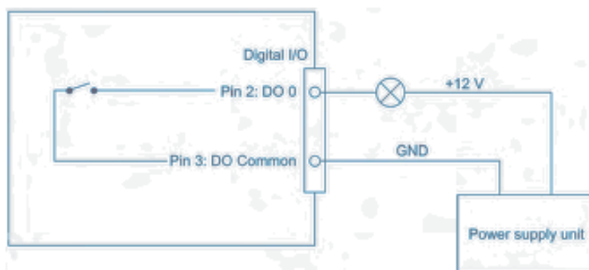
Figure 5-8 Circuit example 2: Digital output
