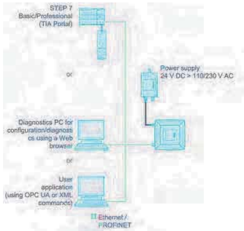
Figure 5-5 Overview: Configuration of RF610R readers
