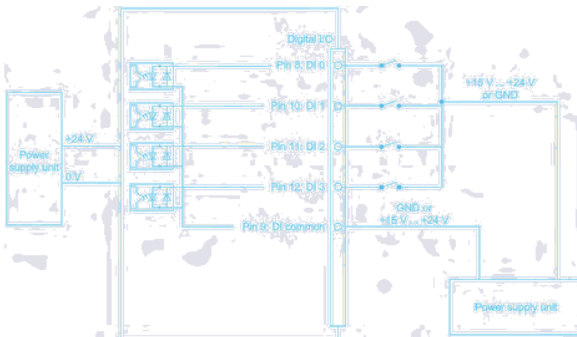
Figure 5-26 Circuit example 2: Digital inputs
