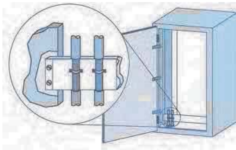
Figure 4-21 Cable shielding
