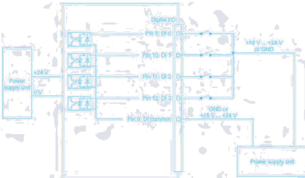
Figure 5-35 Circuit example 2: Digital inputs
