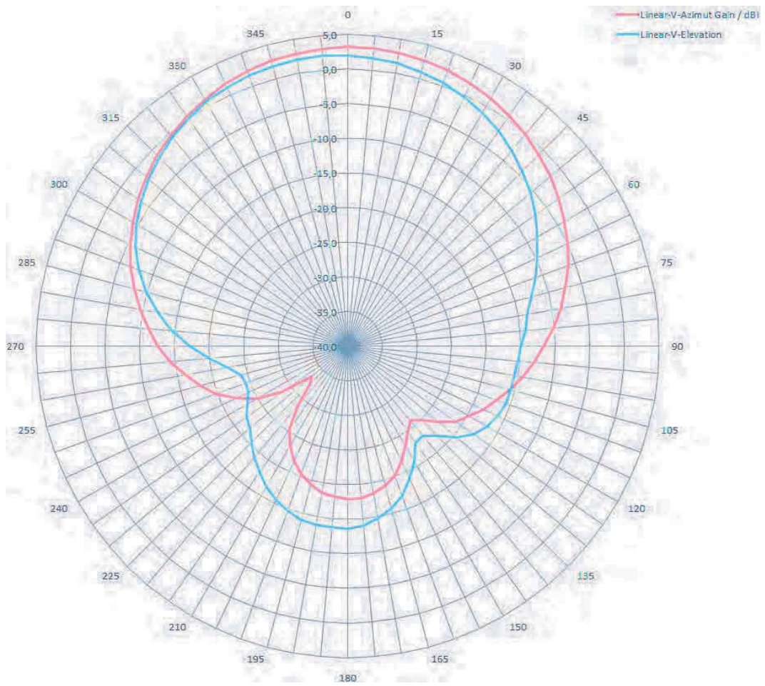
Figure 5-45 Azimuth section
