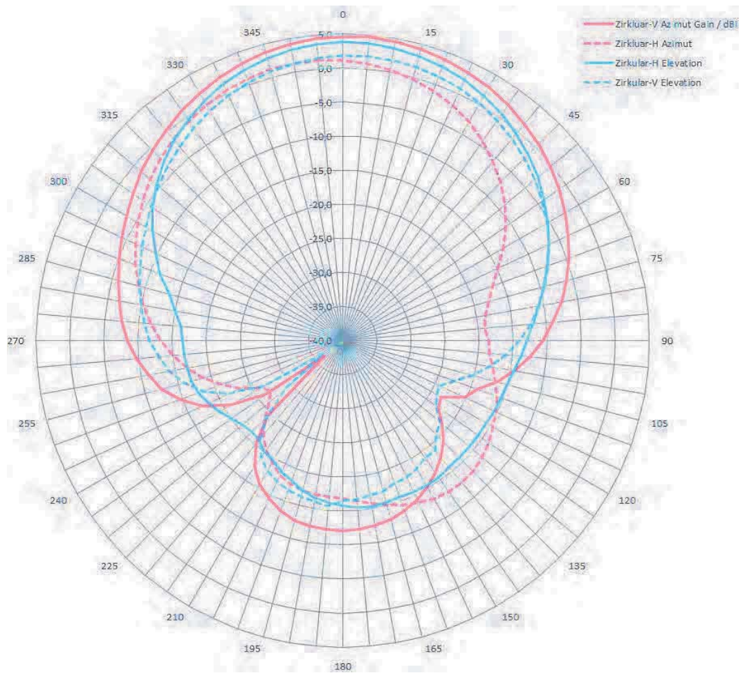
Figure 5-43 Circular section
