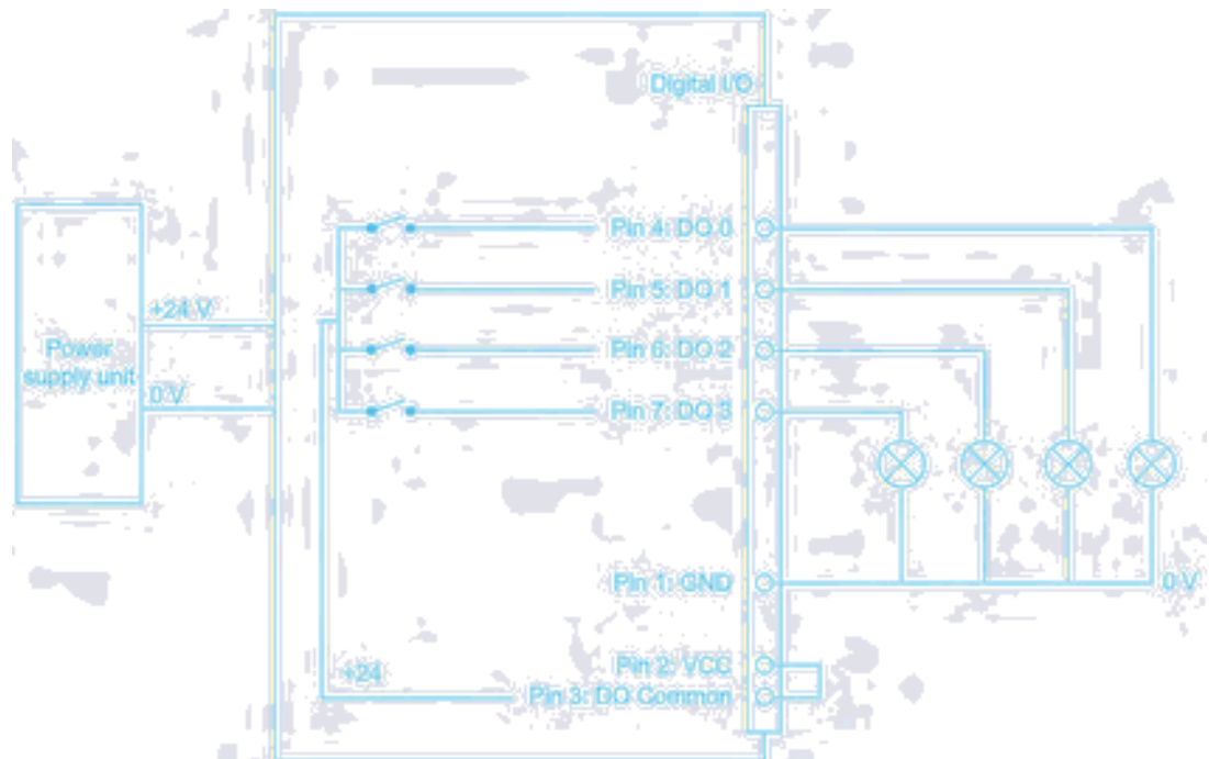
Figure 5-19 Circuit example 4: Digital outputs
