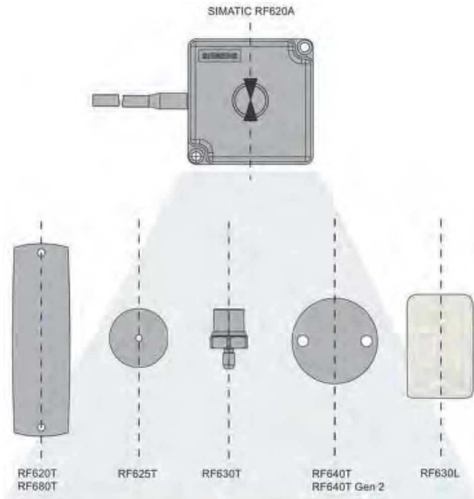
Figure 6-14 Antenna/transponder alignment
