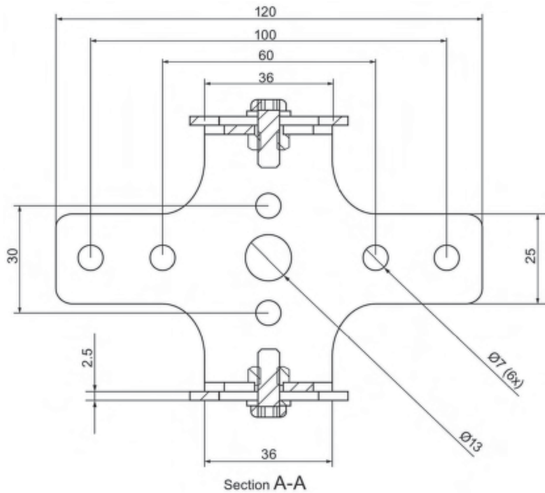
Figure 10-7 Section A-A
