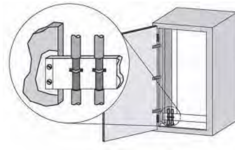
Figure 4-21 Cable shielding
