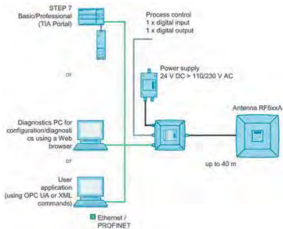
Figure 5-13 Overview: Configuration of RF615R readers
