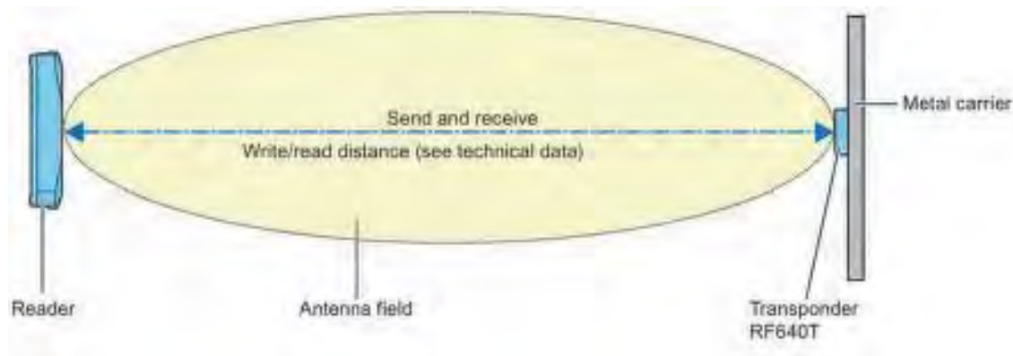
Figure 7-26 Example of optimum antenna/transponder positioning with RF600 readers and an RF600 antenna
