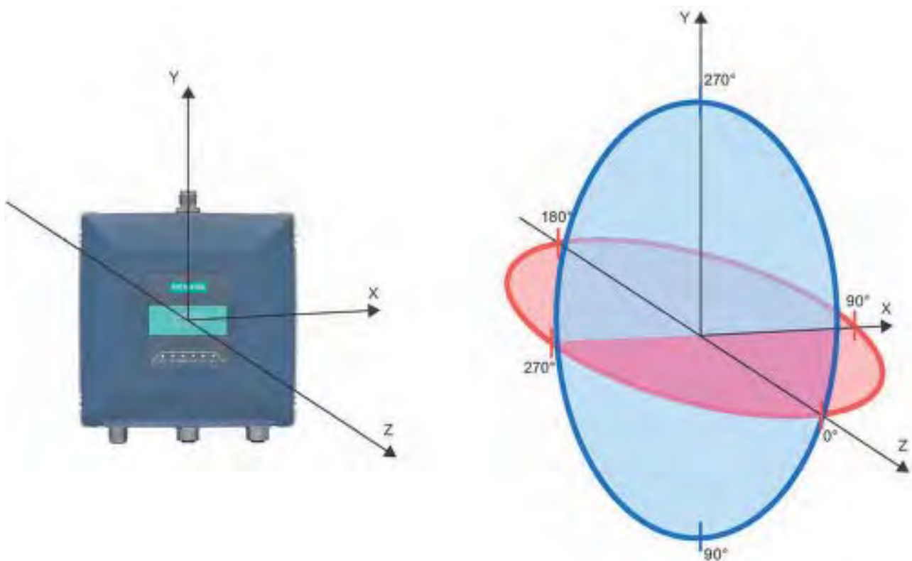
Figure 5-11 Reference system
