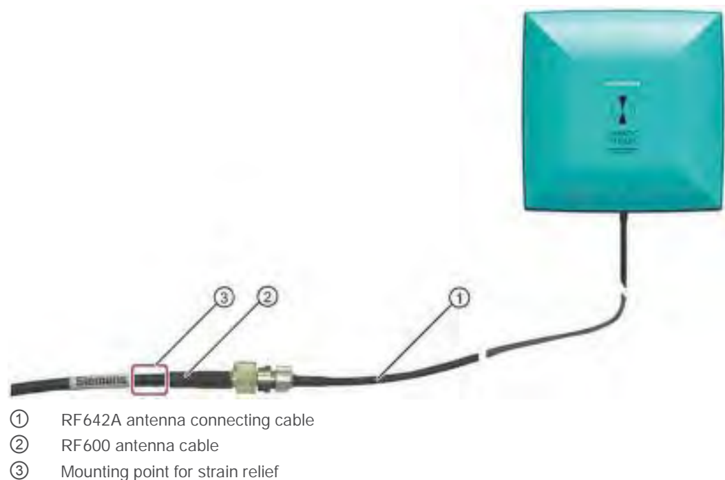
Figure 6-31 Strain relief
