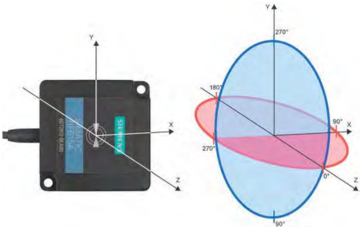
Figure 6-5 Reference system
