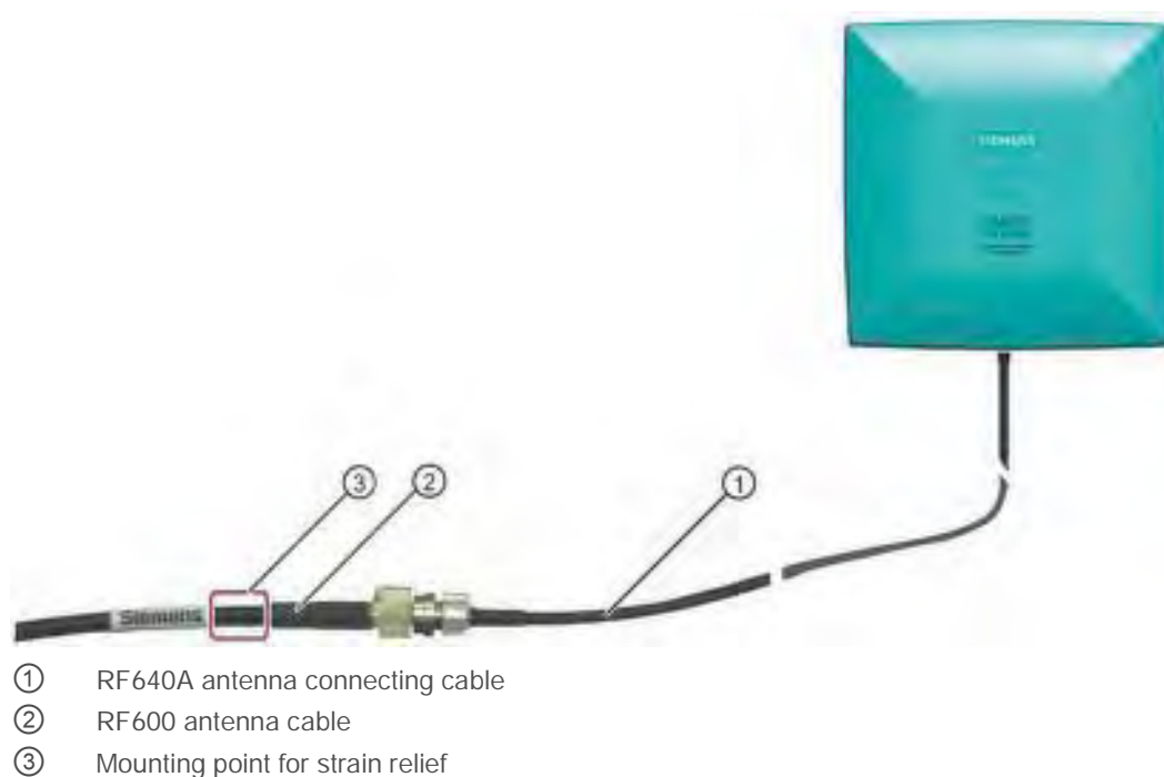
Figure 6-23 Strain relief
