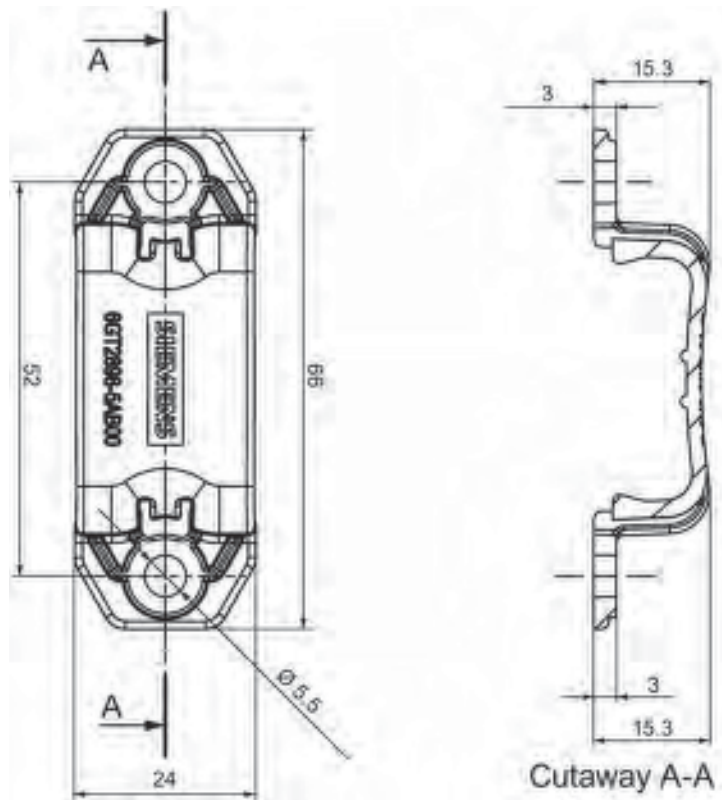
Figure 7-33 Dimension drawing (6GT2898-5AB00) for SIMATIC RF645T
