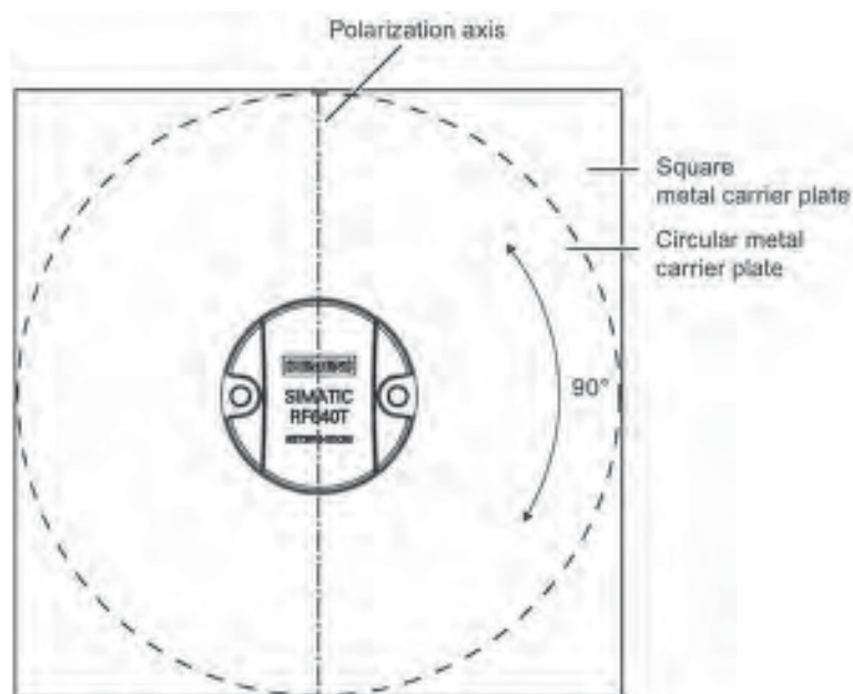
Figure 7-27 Optimum positioning of the transponder on a (square or circular) metal surface
