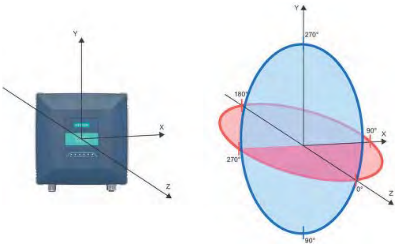
Figure 5-3 Reference system
