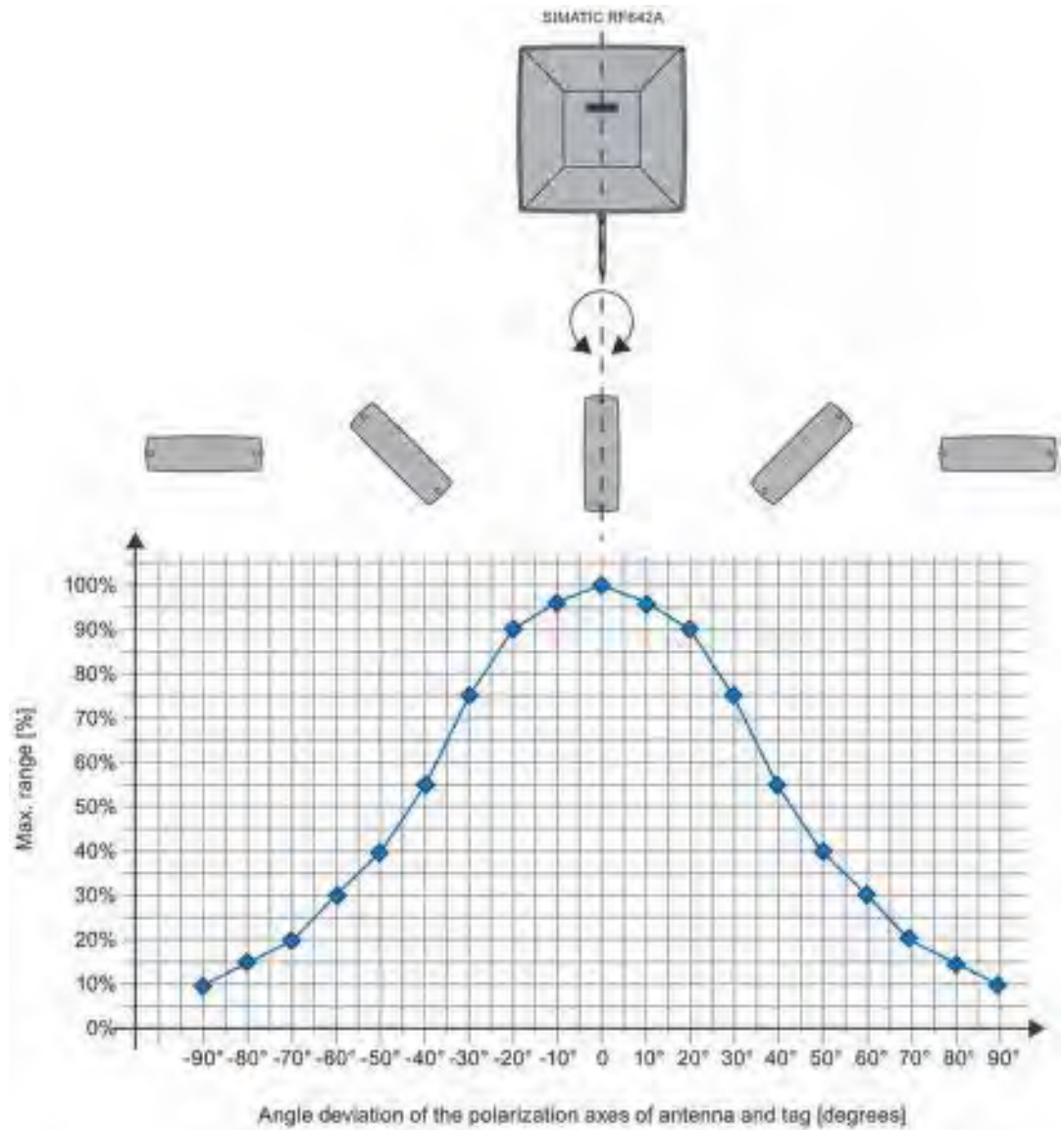
Figure 6-34 Angle deviation diagram for alignment
