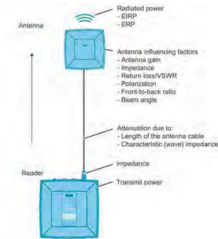
Figure 4-9 Overview diagram: Influencing factors
