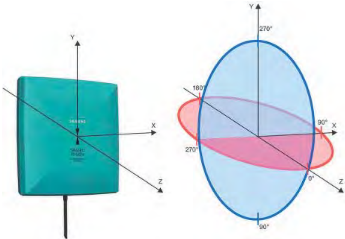
Figure 6-37 Reference system
