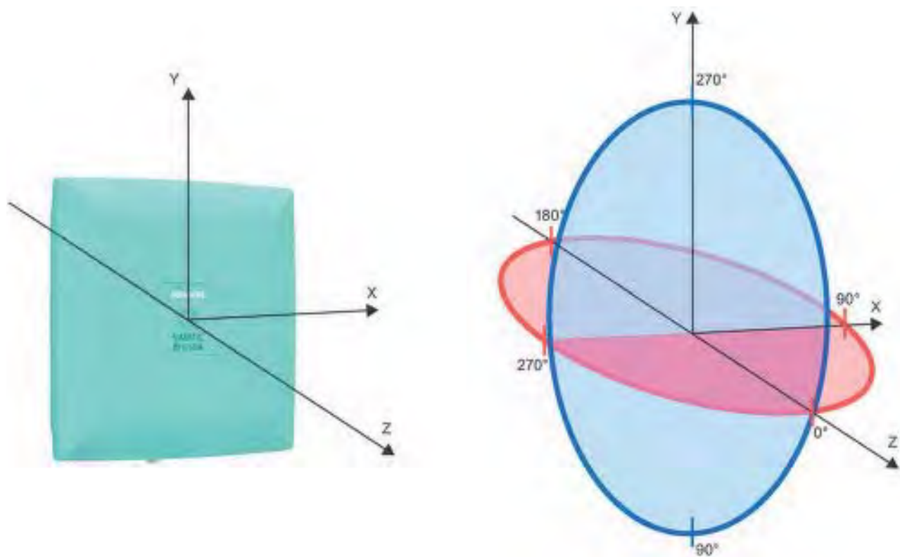
Figure 6-42 Reference system
