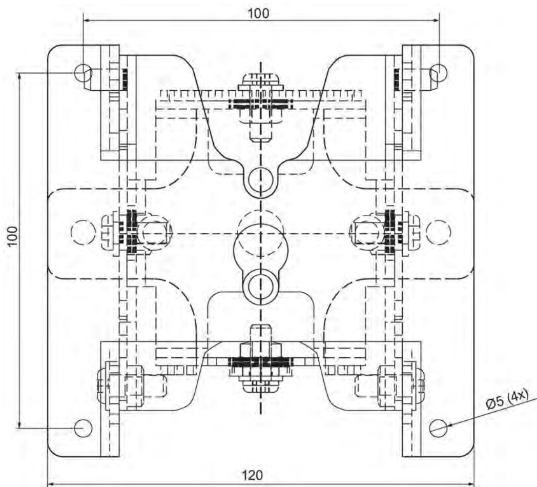
Figure 10-5 Front view
