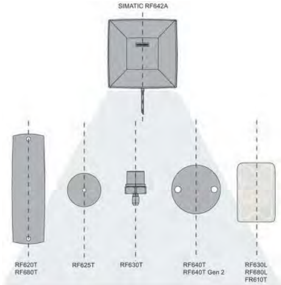
Figure 6-33 Antenna/transponder alignment
