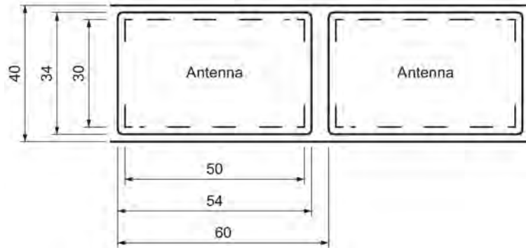
Figure 7-6 Dimension drawing SIMATIC RF630L (6GT2810-2AB03)
