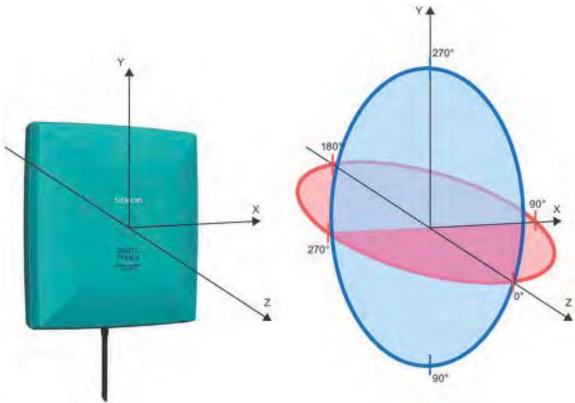
Figure 6-24 Reference system
