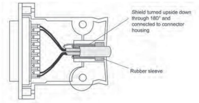
Figure 4-23 Interruption of shielded cables
