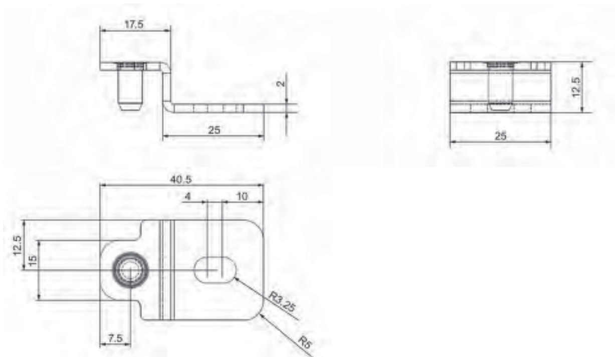
Figure 7-42 Dimension drawing mounting for SIMATIC RF68xT
