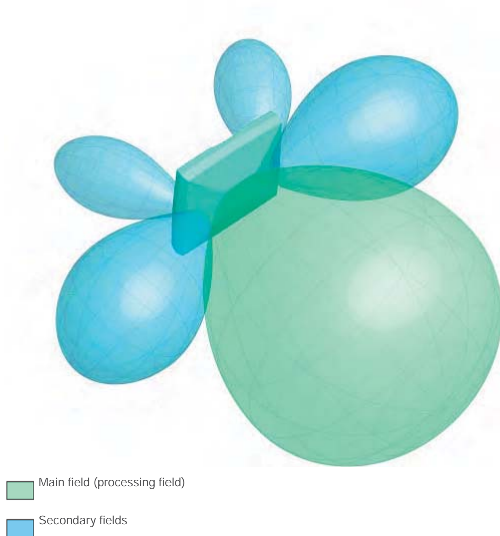
Figure 6-48 Main and auxiliary fields of the RF660A antenna
