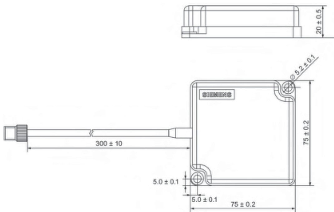
Figure 6-22 Dimension drawing RF620A
