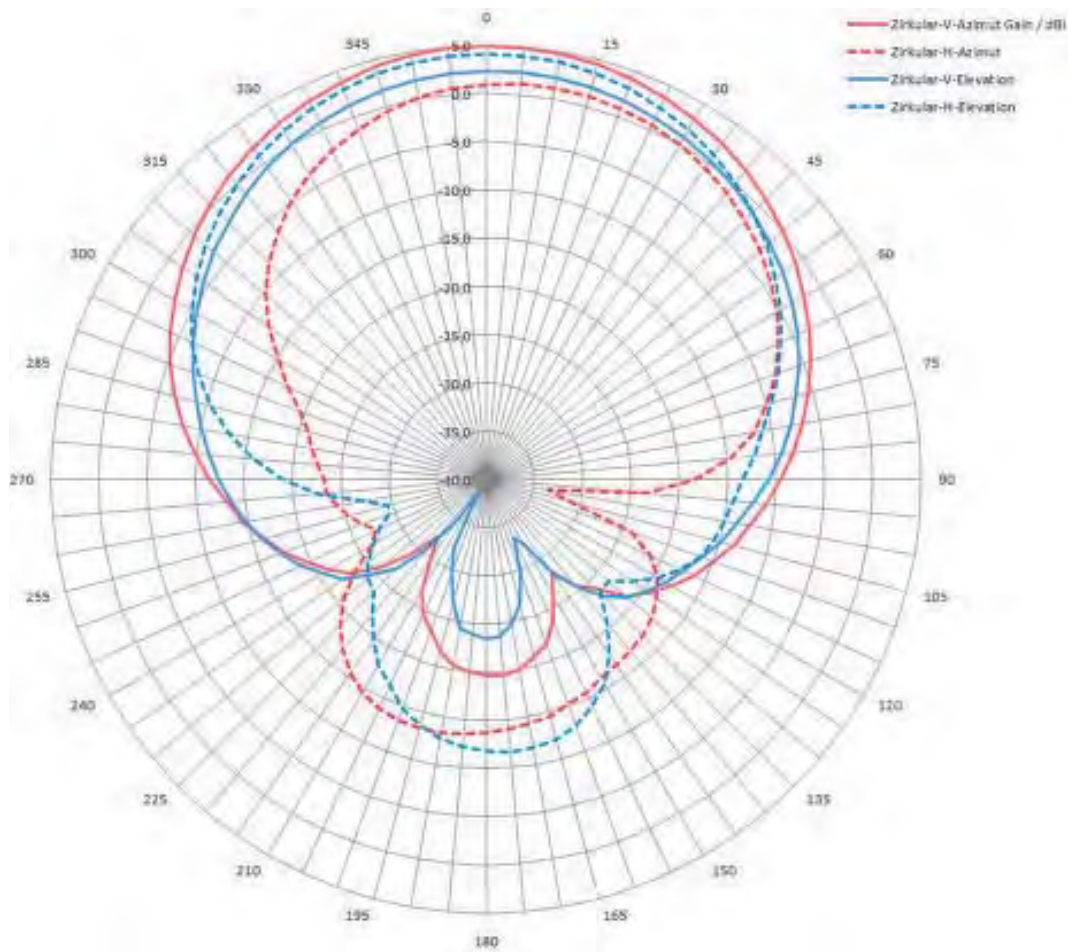
Figure 5-47 Circular section
