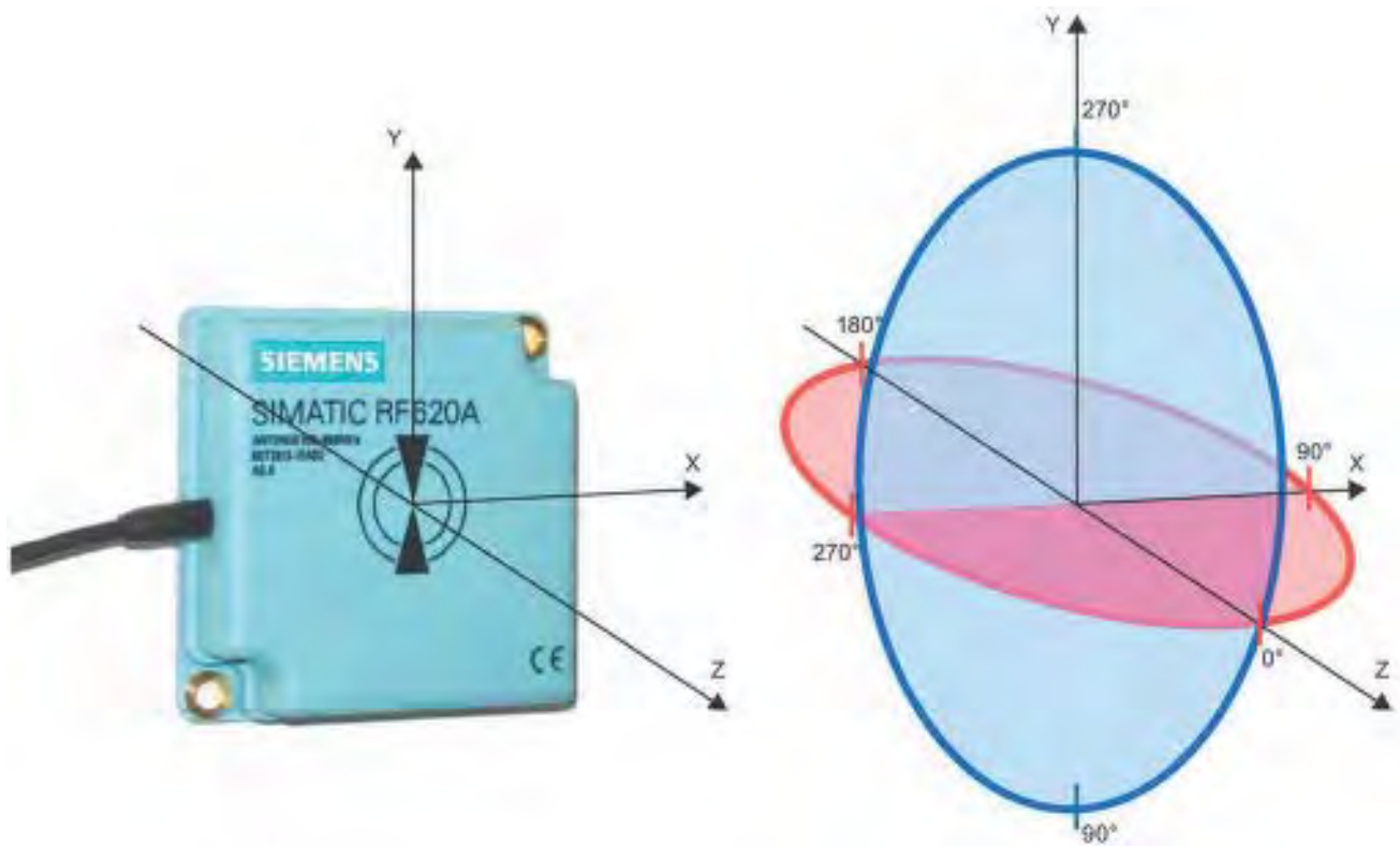
Figure 6-19 Reference system
