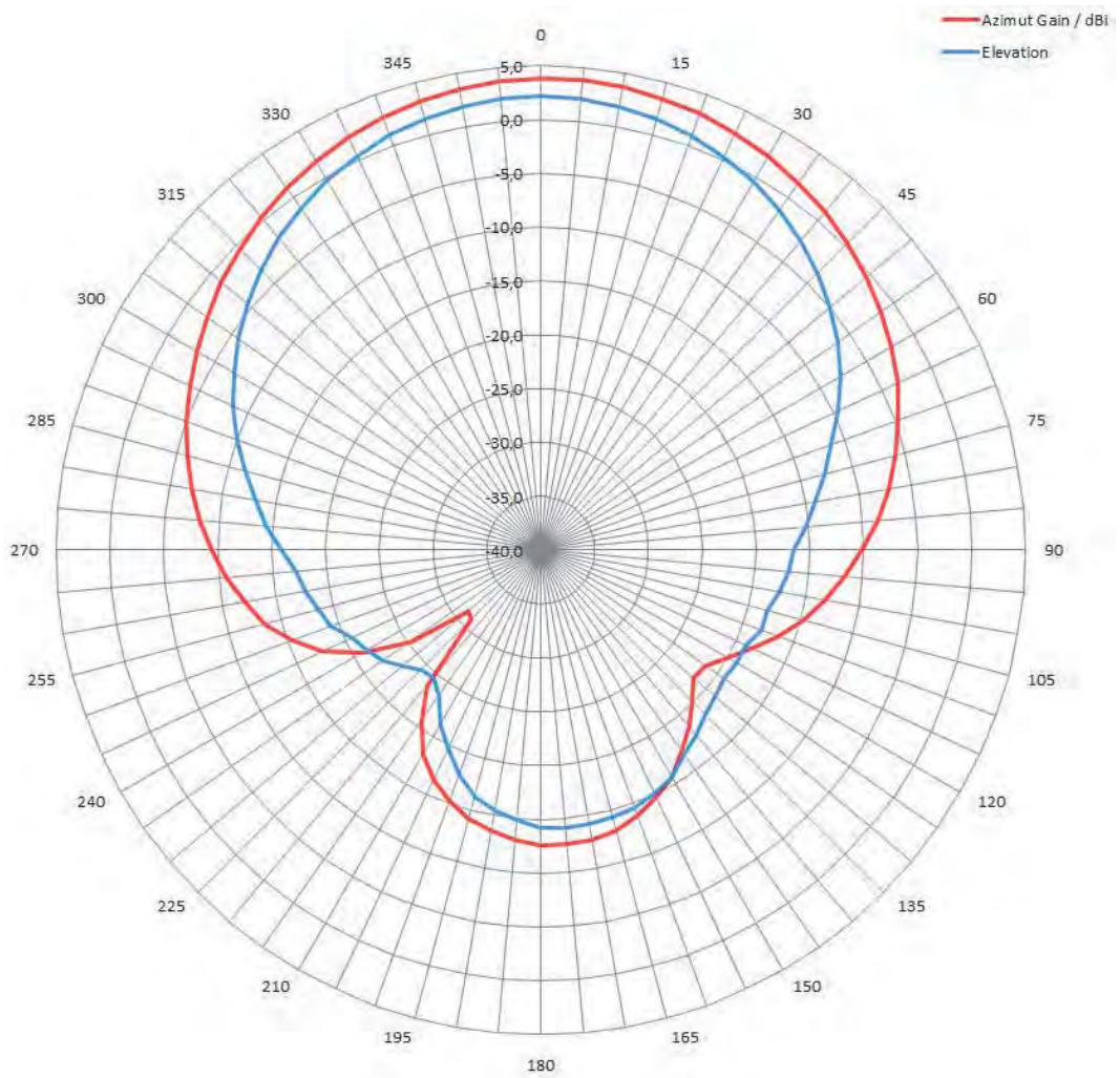
Figure 5-41 Azimuth section
