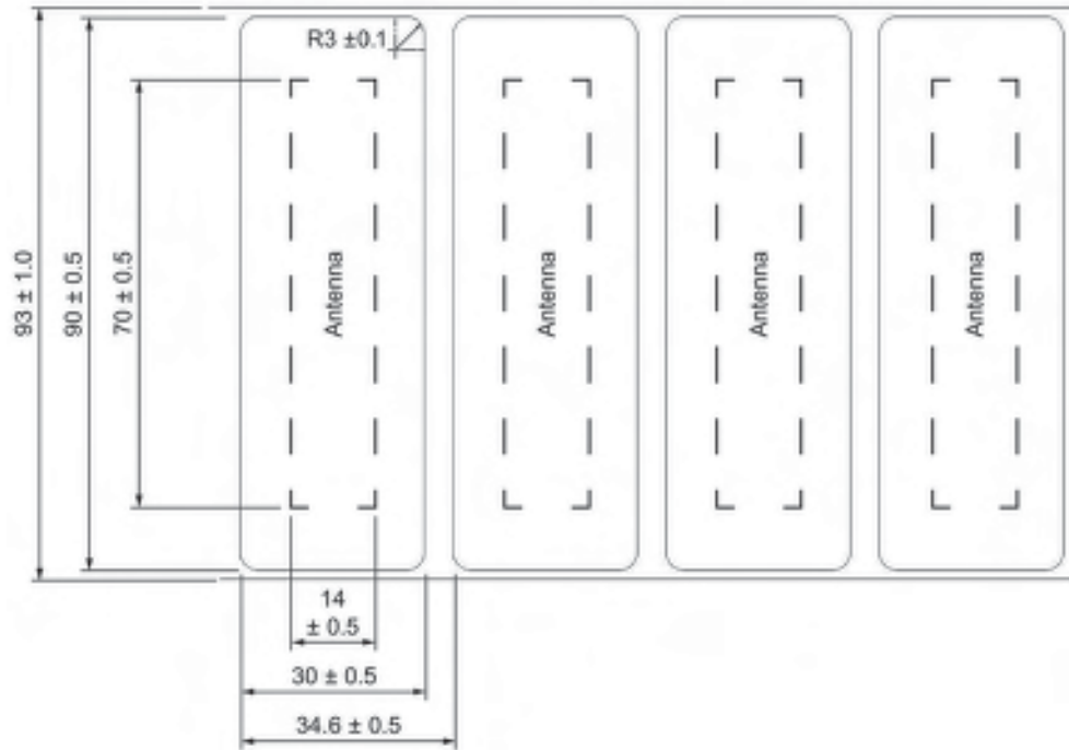
Figure 7-10 Dimension drawing SIMATIC RF630L (6GT2810-2AE81-0AX1)
