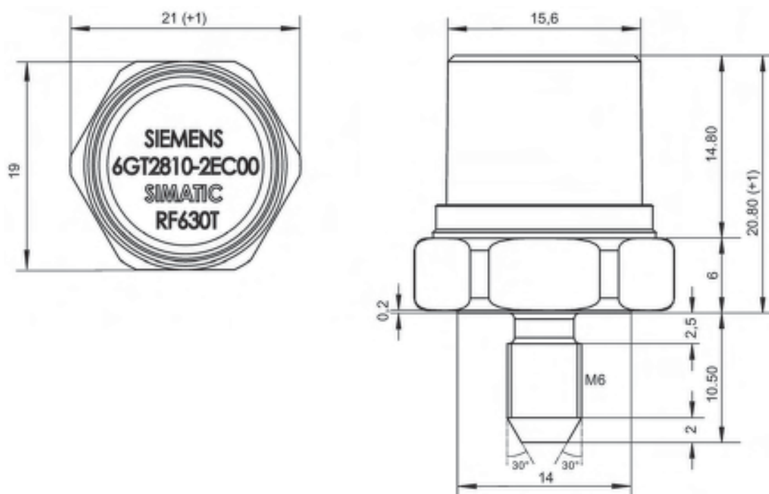
Figure 7-25 SIMATIC RF630T
