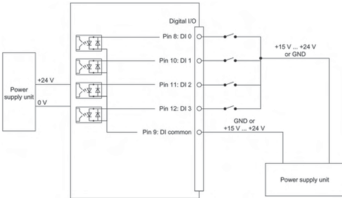
Figure 5-26 Circuit example 2: Digital inputs
