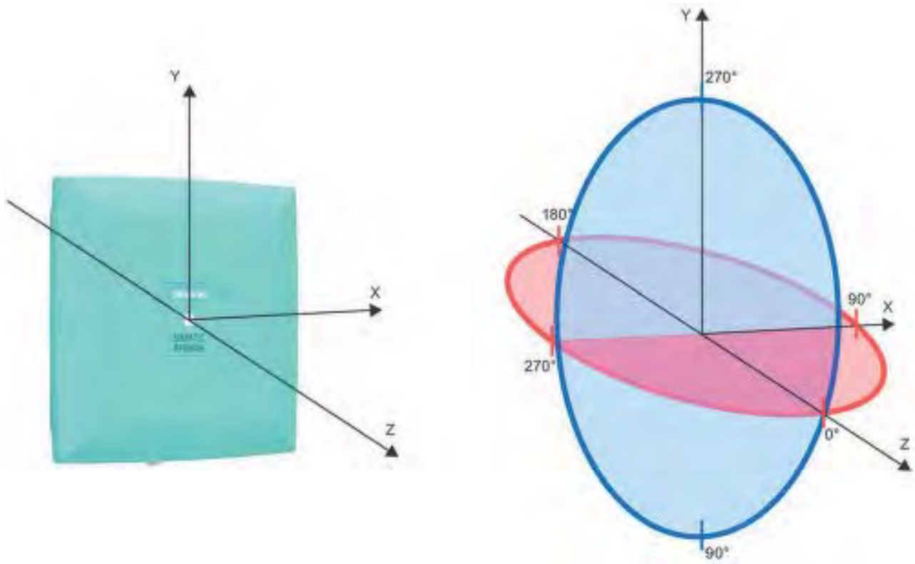
Figure 6-59 Reference system
