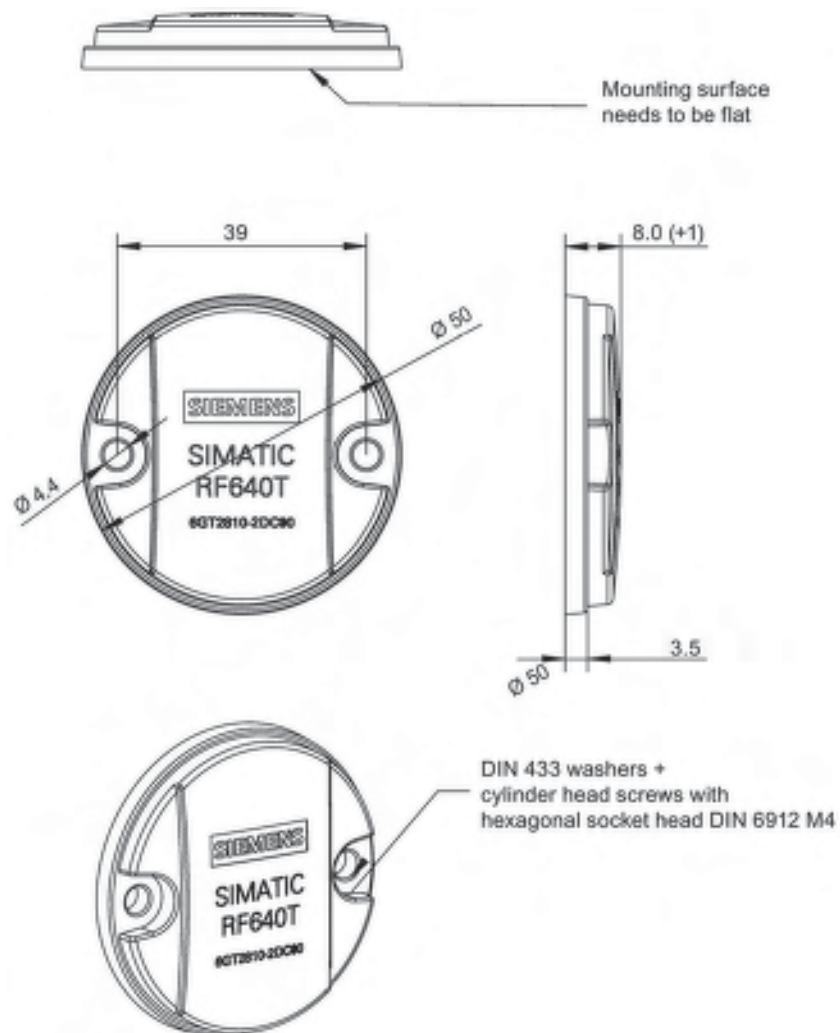
Figure 7-30 SIMATIC RF640T
