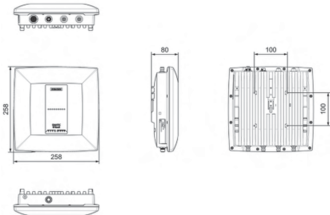
Figure 5-49 Dimension drawing RF685R
