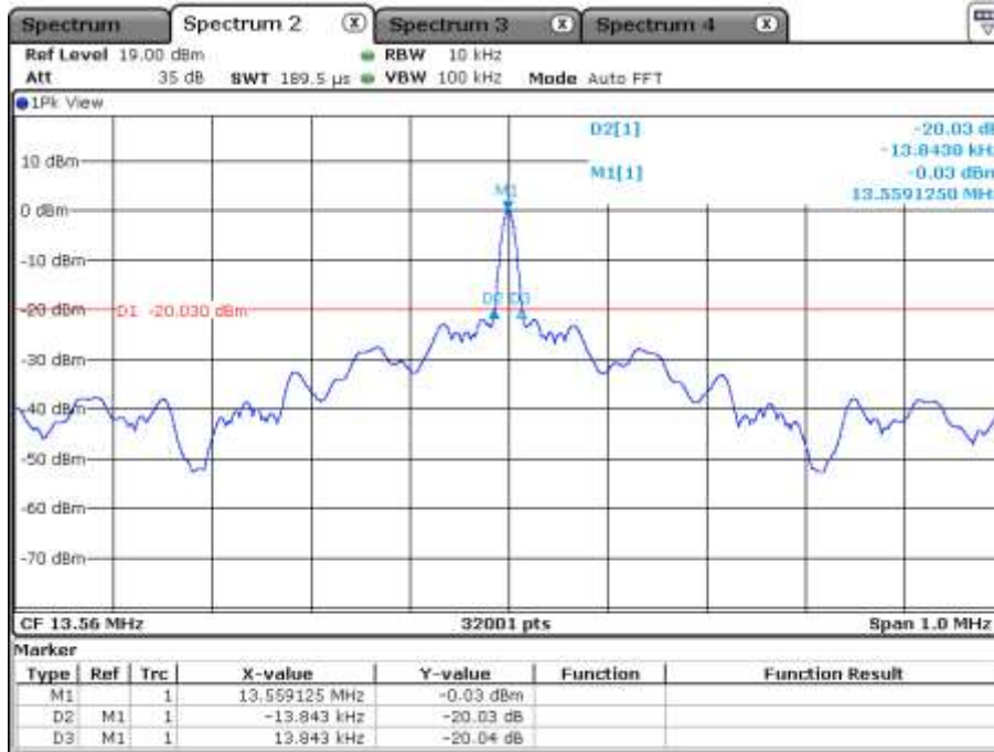
Figure 1 - 20 dB Bandwidth
