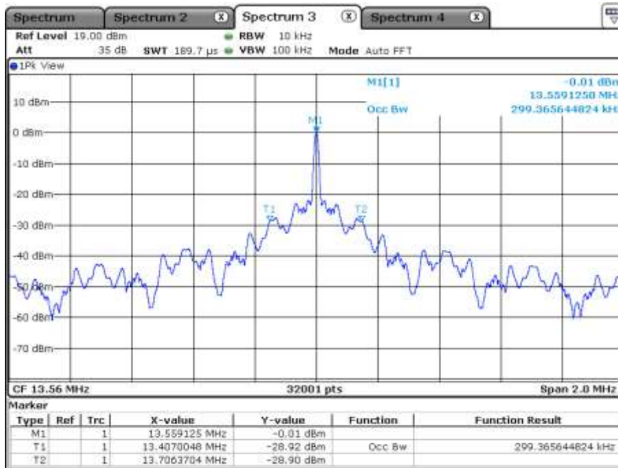
Figure 2 - 99% Occupied Bandwidth
