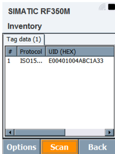
Figure 6-2 "Tag Data" tab in the "Inventory" menu
