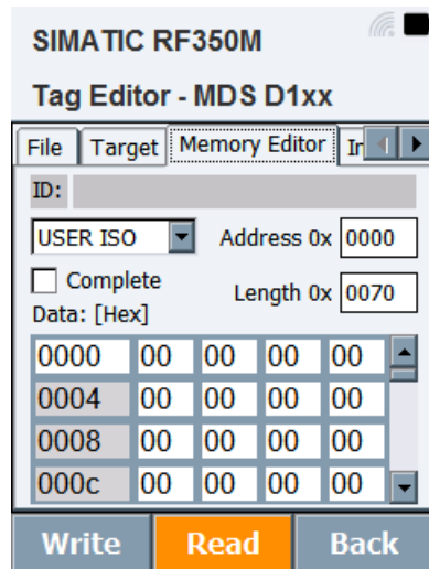
Figure 6-6 "Memory Editor" tab in the "Tag Editor" menu
