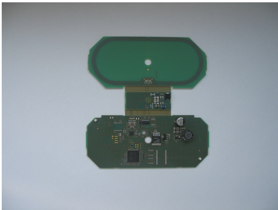
Fig. 1: PCB Side A RF280R (RS422)
